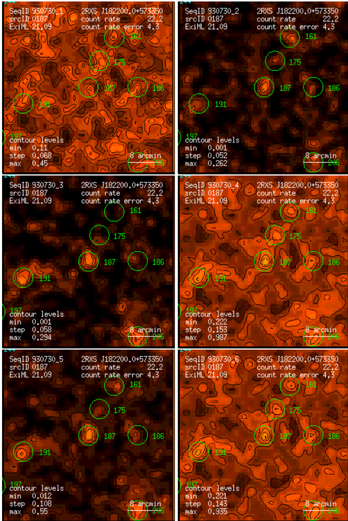
Figure 187: RASS 930730: detection 0187: band rate images, Gaussian filter: (1) PSPC channels 11 – 41, (2) 52 – 90, (3) 91 – 201, (4) 11 – 235, (5) 52 – 201, (6) 11 – 201. Broad band rates in counts/ks. Band rate contour levels in counts/ks/arcmin 2 .
