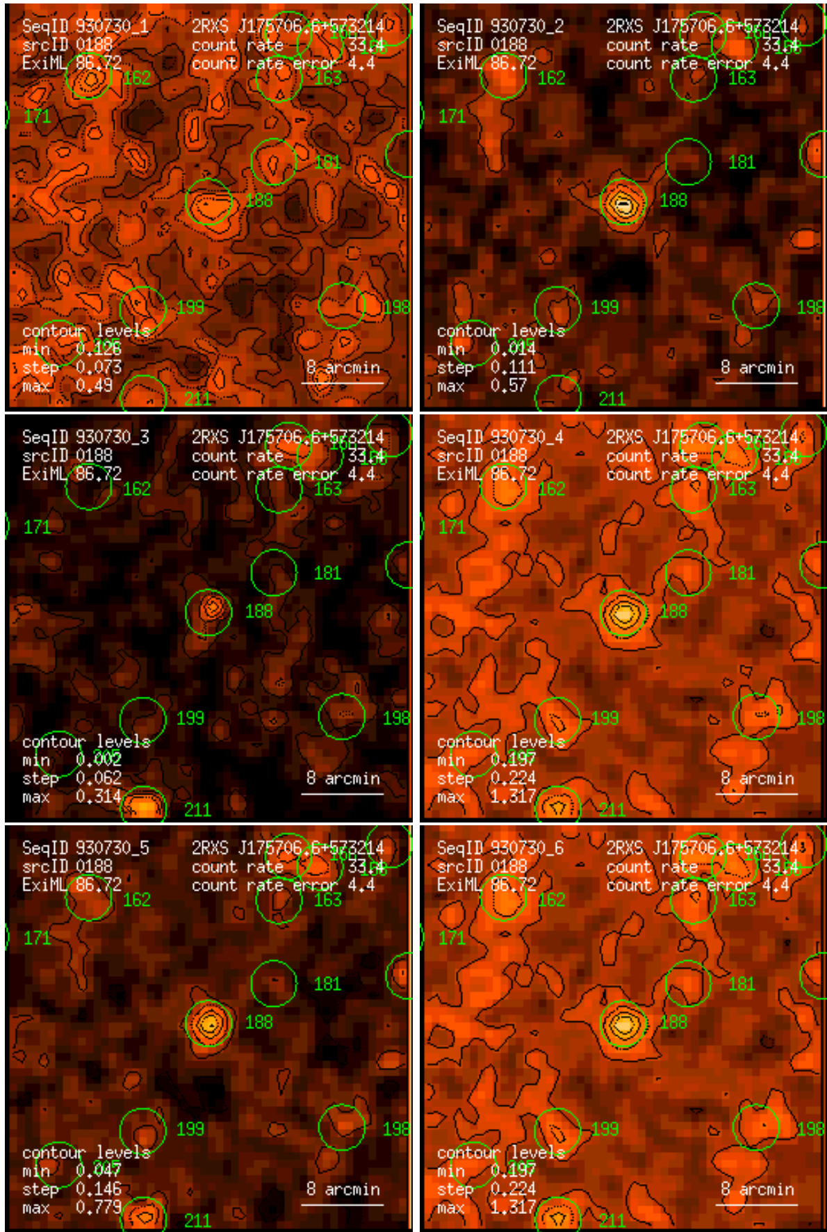
Figure 188: RASS 930730: detection 0188: band rate images, Gaussian filter: (1) PSPC channels 11 – 41, (2) 52 – 90, (3) 91 – 201, (4) 11 – 235, (5) 52 – 201, (6) 11 – 201. Broad band rates in counts/ks. Band rate contour levels in counts/ks/arcmin 2 .
