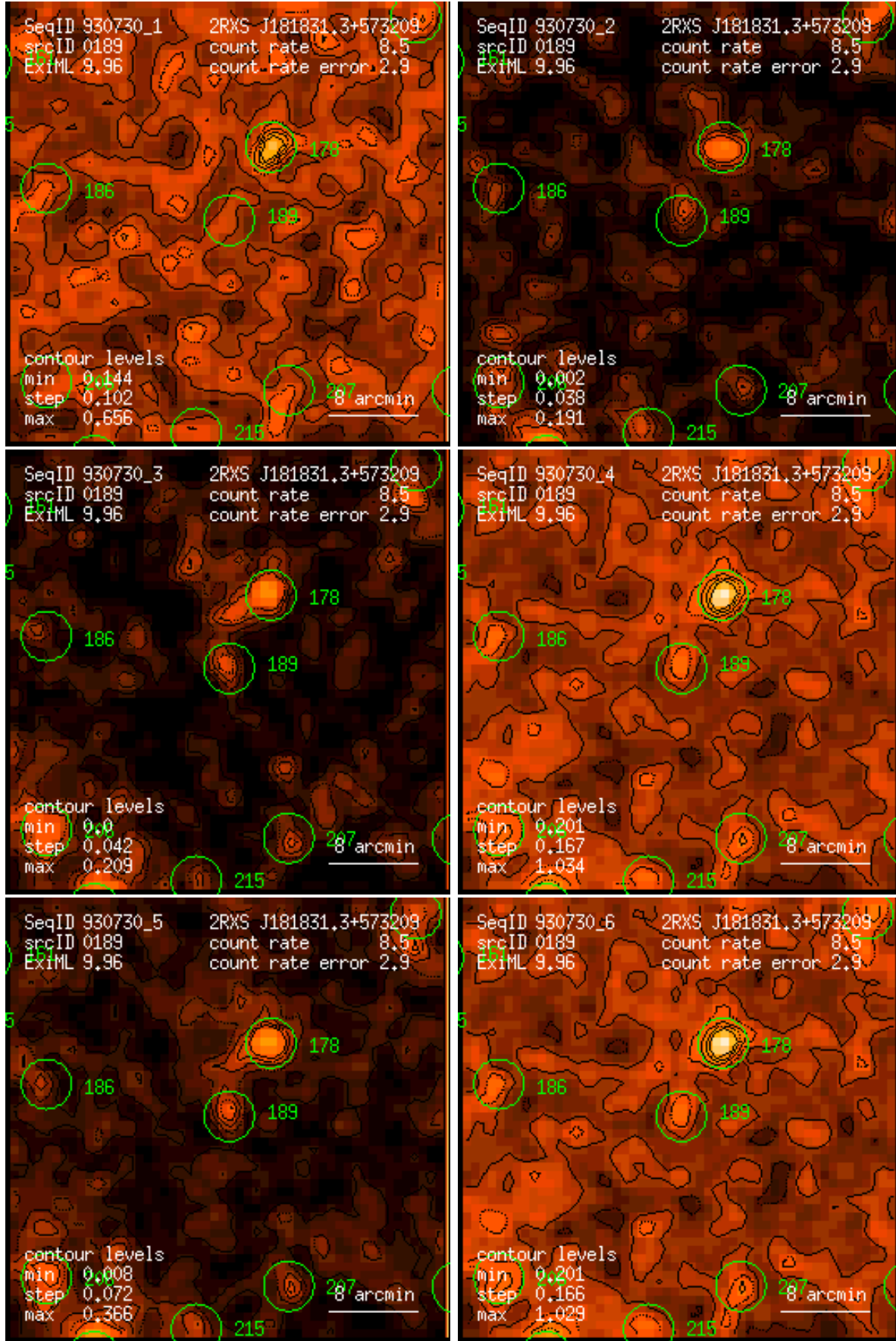
Figure 189: RASS 930730: detection 0189: band rate images, Gaussian filter: (1) PSPC channels 11 – 41, (2) 52 – 90, (3) 91 – 201, (4) 11 – 235, (5) 52 – 201, (6) 11 – 201. Broad band rates in counts/ks. Band rate contour levels in counts/ks/arcmin 2 .
