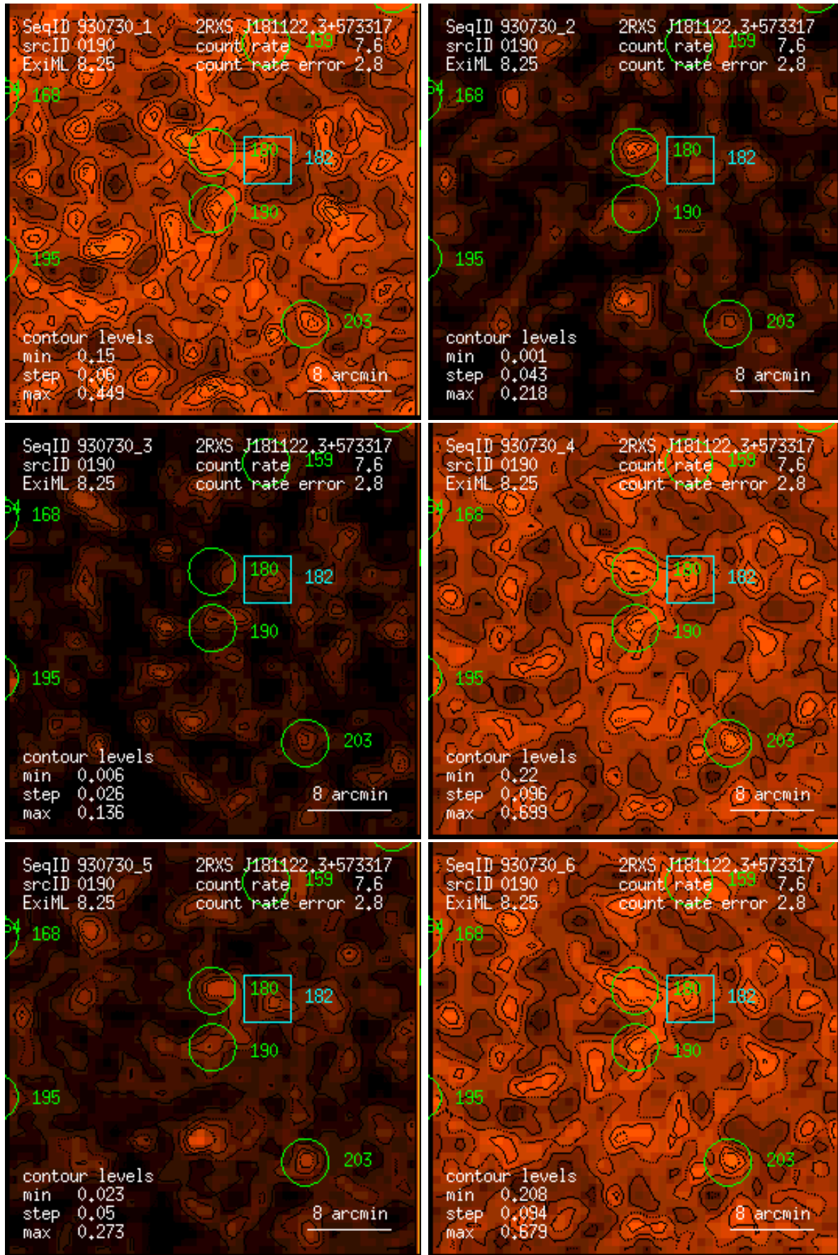
Figure 190: RASS 930730: detection 0190: band rate images, Gaussian filter: (1) PSPC channels 11 – 41, (2) 52 – 90, (3) 91 – 201, (4) 11 – 235, (5) 52 – 201, (6) 11 – 201. Broad band rates in counts/ks. Band rate contour levels in counts/ks/arcmin 2 .
