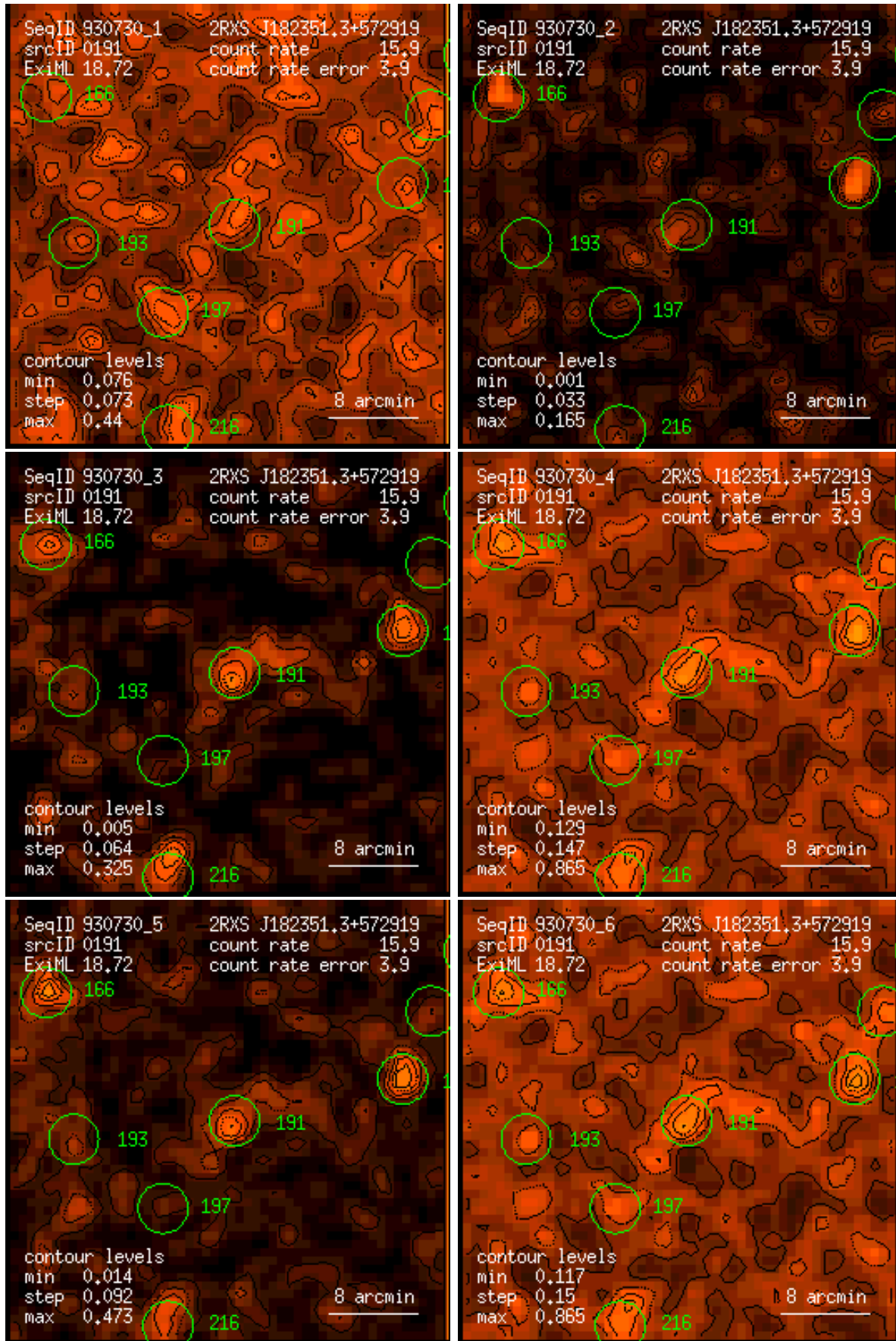
Figure 191: RASS 930730: detection 0191: band rate images, Gaussian filter: (1) PSPC channels 11 – 41, (2) 52 – 90, (3) 91 – 201, (4) 11 – 235, (5) 52 – 201, (6) 11 – 201. Broad band rates in counts/ks. Band rate contour levels in counts/ks/arcmin 2 .
