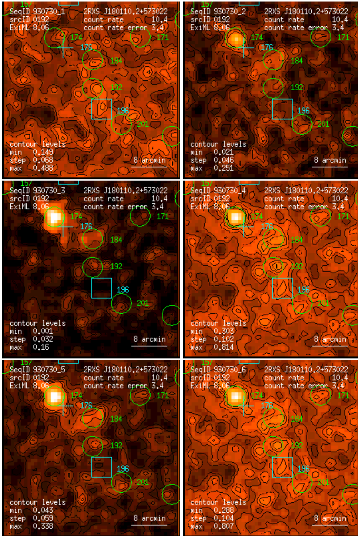
Figure 192: RASS 930730: detection 0192: band rate images, Gaussian filter: (1) PSPC channels 11 – 41, (2) 52 – 90, (3) 91 – 201, (4) 11 – 235, (5) 52 – 201, (6) 11 – 201. Broad band rates in counts/ks. Band rate contour levels in counts/ks/arcmin 2 .
