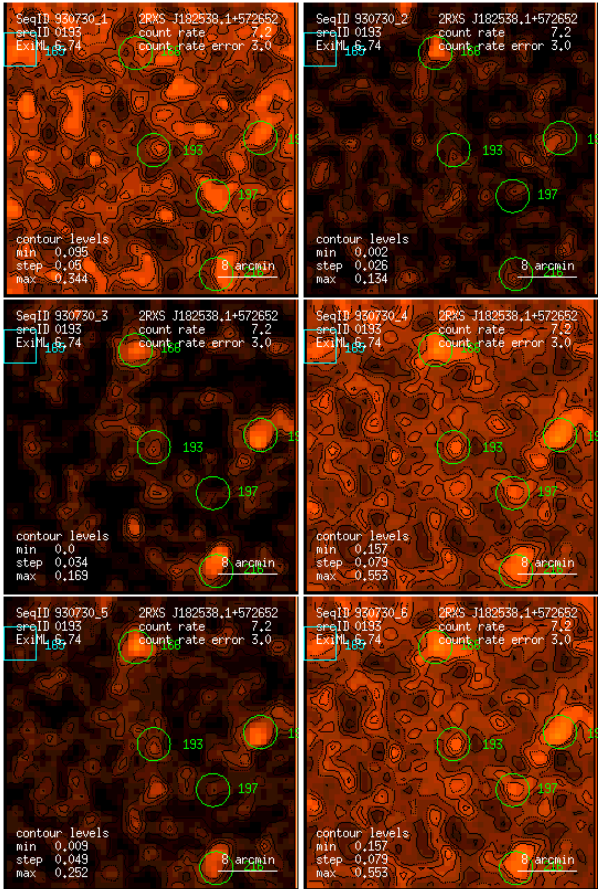
Figure 193: RASS 930730: detection 0193: band rate images, Gaussian filter: (1) PSPC channels 11 – 41, (2) 52 – 90, (3) 91 – 201, (4) 11 – 235, (5) 52 – 201, (6) 11 – 201. Broad band rates in counts/ks. Band rate contour levels in counts/ks/arcmin 2 .
