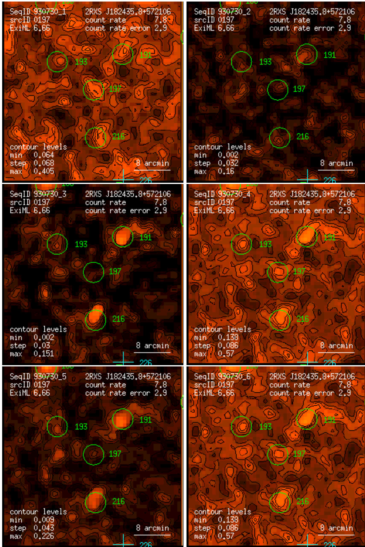
Figure 197: RASS 930730: detection 0197: band rate images, Gaussian filter: (1) PSPC channels 11 – 41, (2) 52 – 90, (3) 91 – 201, (4) 11 – 235, (5) 52 – 201, (6) 11 – 201. Broad band rates in counts/ks. Band rate contour levels in counts/ks/arcmin 2 .
