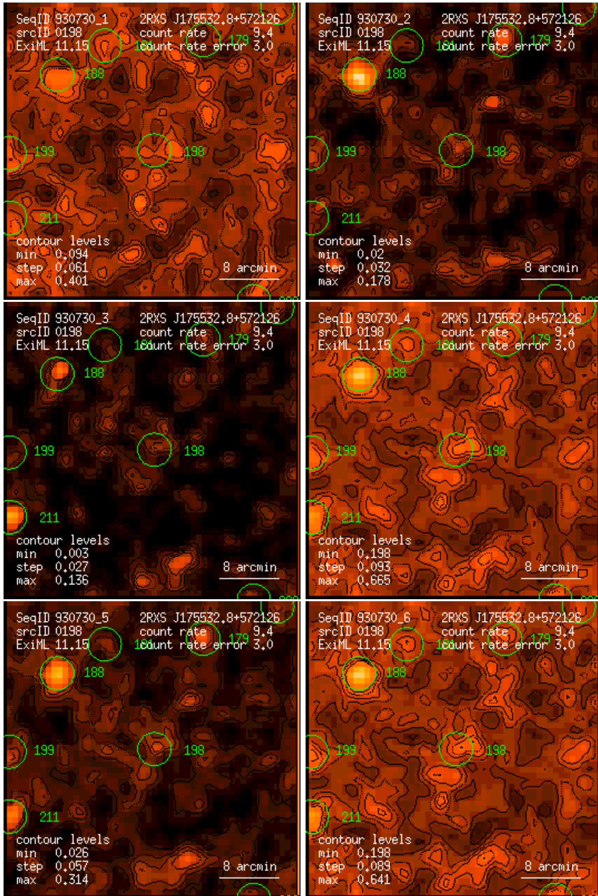
Figure 198: RASS 930730: detection 0198: band rate images, Gaussian filter: (1) PSPC channels 11 – 41, (2) 52 – 90, (3) 91 – 201, (4) 11 – 235, (5) 52 – 201, (6) 11 – 201. Broad band rates in counts/ks. Band rate contour levels in counts/ks/arcmin 2 .
