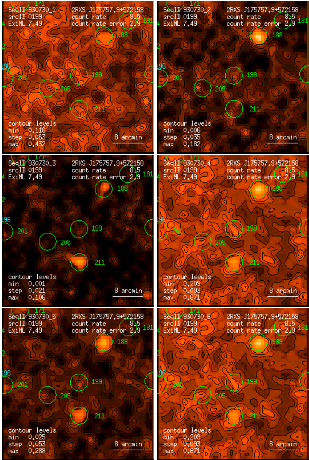
Figure 199: RASS 930730: detection 0199: band rate images, Gaussian filter: (1) PSPC channels 11 – 41, (2) 52 – 90, (3) 91 – 201, (4) 11 – 235, (5) 52 – 201, (6) 11 – 201. Broad band rates in counts/ks. Band rate contour levels in counts/ks/arcmin 2 .
