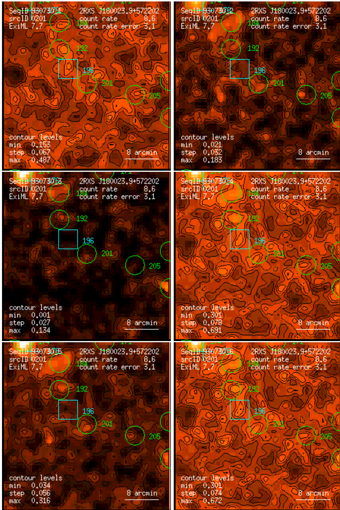
Figure 201: RASS 930730: detection 0201: band rate images, Gaussian filter: (1) PSPC channels 11 – 41, (2) 52 – 90, (3) 91 – 201, (4) 11 – 235, (5) 52 – 201, (6) 11 – 201. Broad band rates in counts/ks. Band rate contour levels in counts/ks/arcmin 2 .
