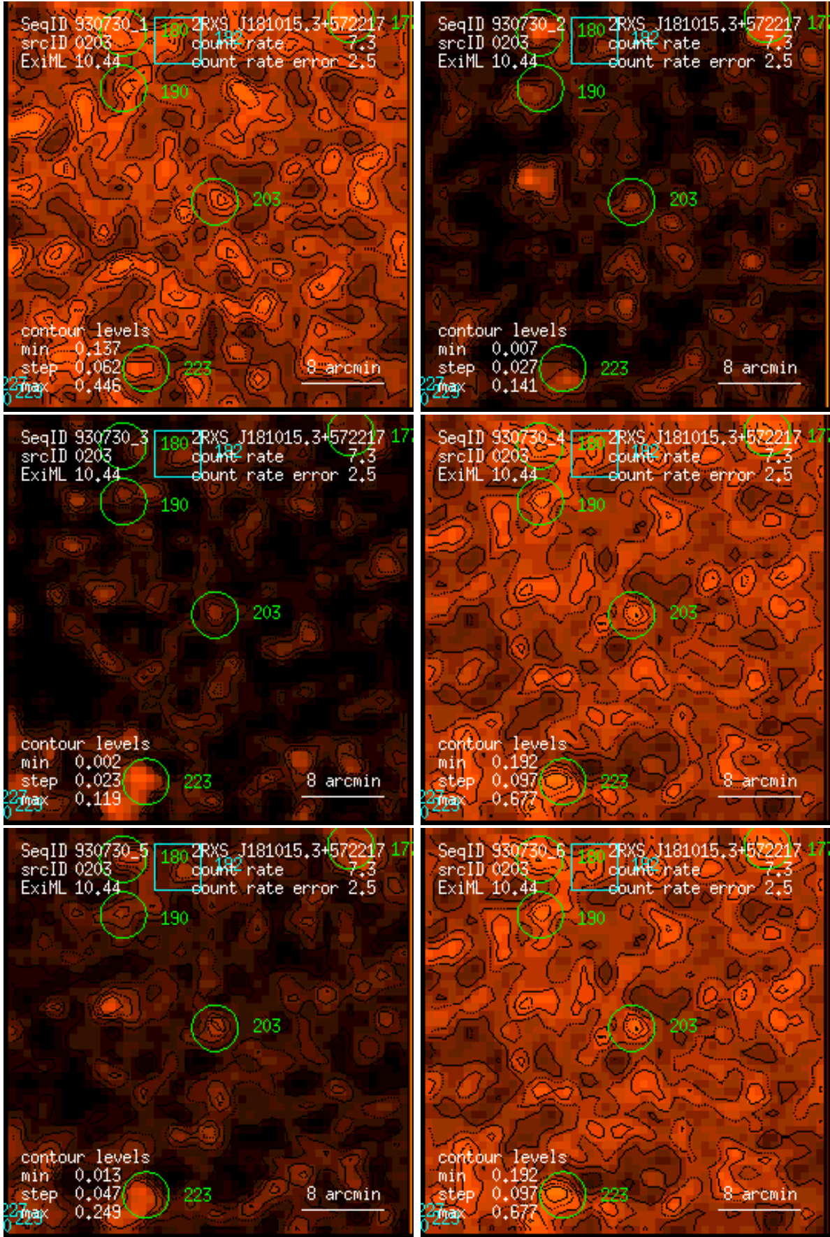
Figure 203: RASS 930730: detection 0203: band rate images, Gaussian filter: (1) PSPC channels 11 – 41, (2) 52 – 90, (3) 91 – 201, (4) 11 – 235, (5) 52 – 201, (6) 11 – 201. Broad band rates in counts/ks. Band rate contour levels in counts/ks/arcmin 2 .
