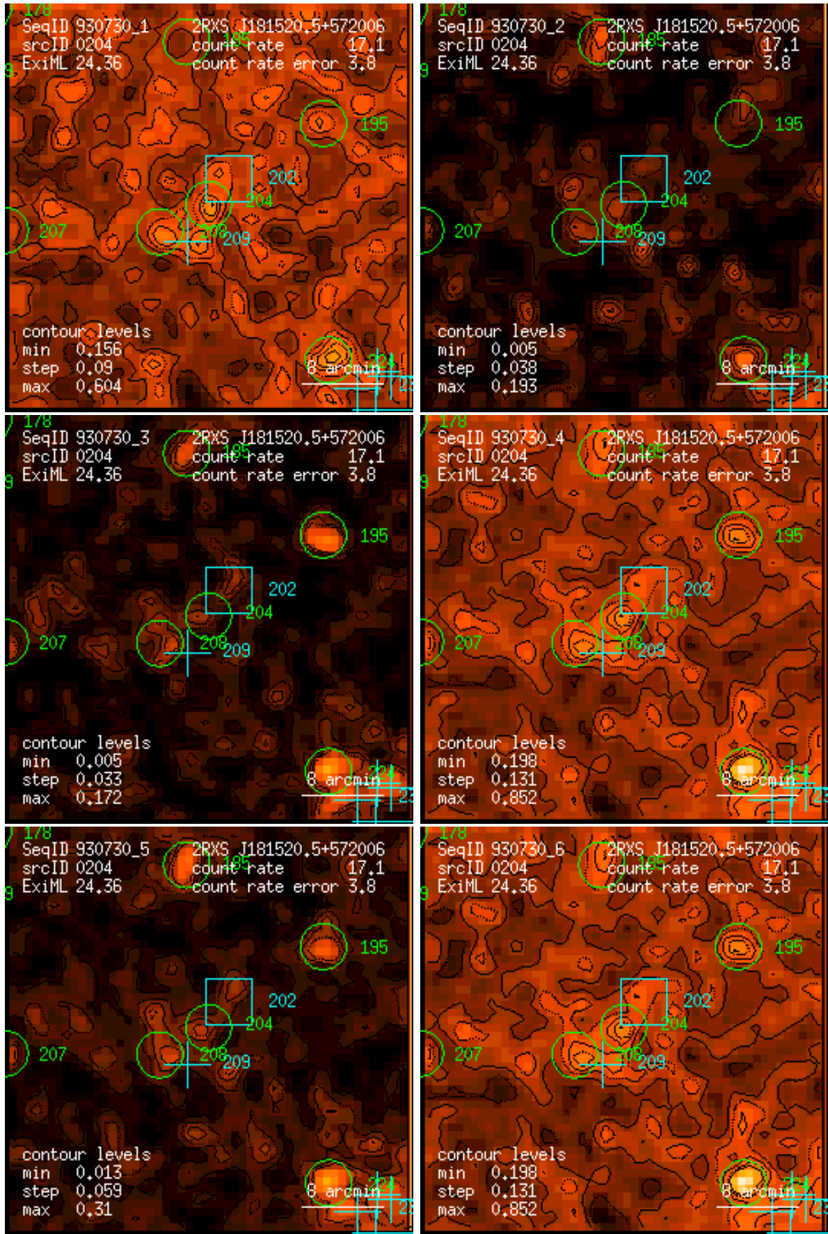
Figure 204: RASS 930730: detection 0204: band rate images, Gaussian filter: (1) PSPC channels 11 – 41, (2) 52 – 90, (3) 91 – 201, (4) 11 – 235, (5) 52 – 201, (6) 11 – 201. Broad band rates in counts/ks. Band rate contour levels in counts/ks/arcmin 2 .
