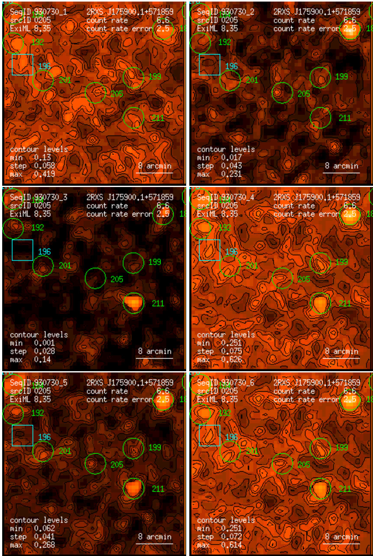
Figure 205: RASS 930730: detection 0205: band rate images, Gaussian filter: (1) PSPC channels 11 – 41, (2) 52 – 90, (3) 91 – 201, (4) 11 – 235, (5) 52 – 201, (6) 11 – 201. Broad band rates in counts/ks. Band rate contour levels in counts/ks/arcmin 2 .
