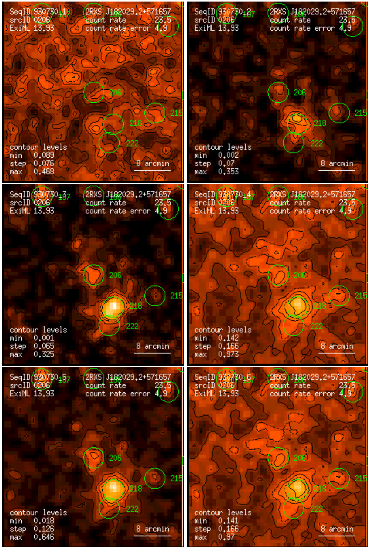
Figure 206: RASS 930730: detection 0206: band rate images, Gaussian filter: (1) PSPC channels 11 – 41, (2) 52 – 90, (3) 91 – 201, (4) 11 – 235, (5) 52 – 201, (6) 11 – 201. Broad band rates in counts/ks. Band rate contour levels in counts/ks/arcmin 2 .
