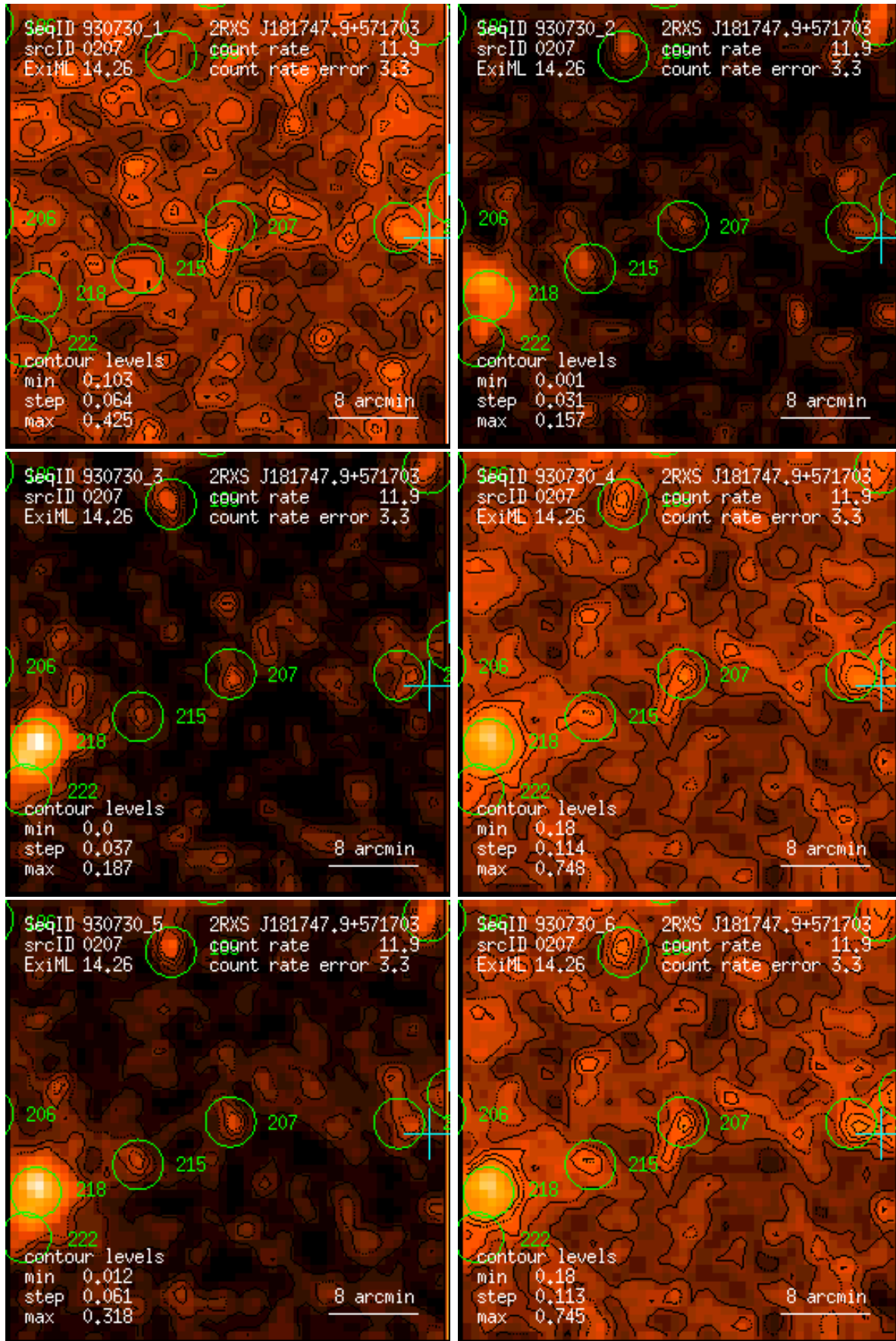
Figure 207: RASS 930730: detection 0207: band rate images, Gaussian filter: (1) PSPC channels 11 – 41, (2) 52 – 90, (3) 91 – 201, (4) 11 – 235, (5) 52 – 201, (6) 11 – 201. Broad band rates in counts/ks. Band rate contour levels in counts/ks/arcmin 2 .
