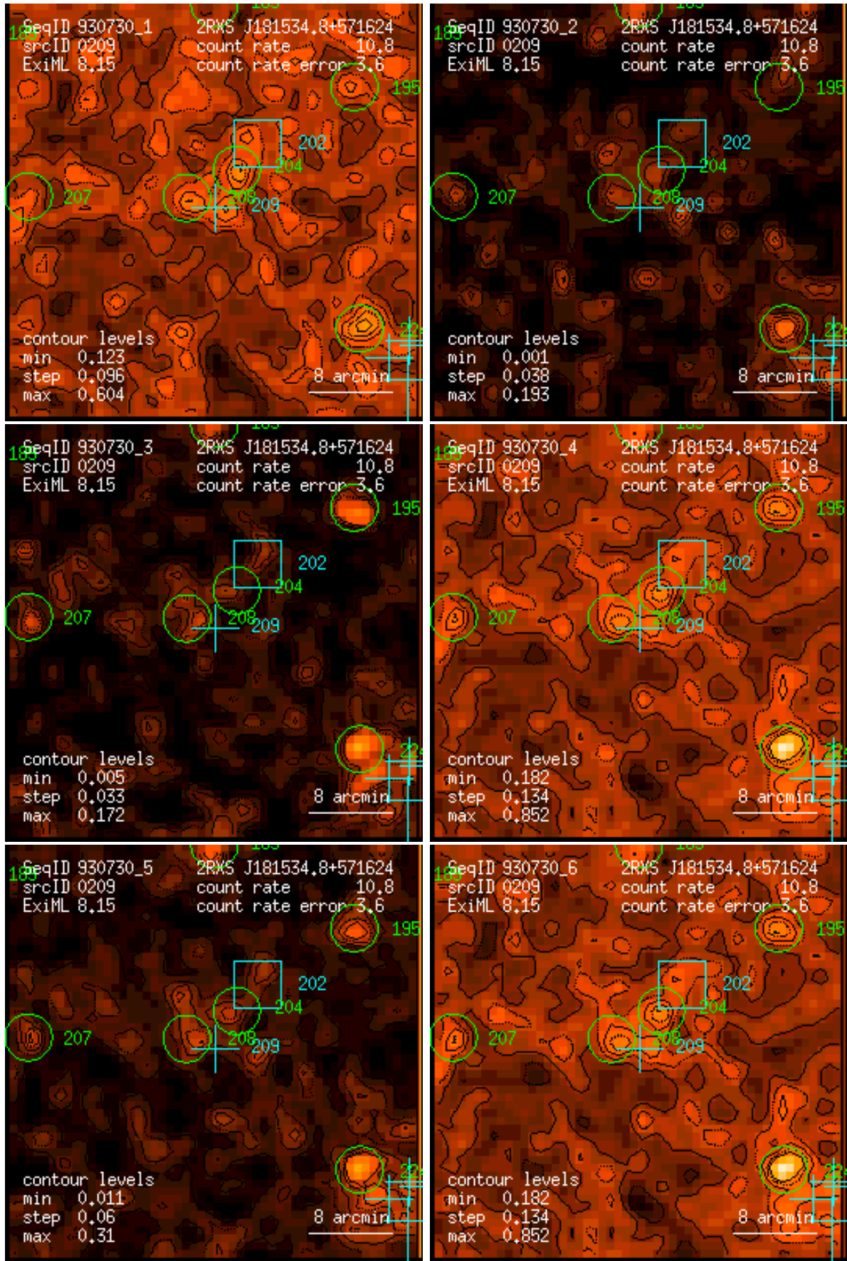
Figure 209: RASS 930730: detection 0209: band rate images, Gaussian filter: (1) PSPC channels 11 – 41, (2) 52 – 90, (3) 91 – 201, (4) 11 – 235, (5) 52 – 201, (6) 11 – 201. Broad band rates in counts/ks. Band rate contour levels in counts/ks/arcmin 2 .
