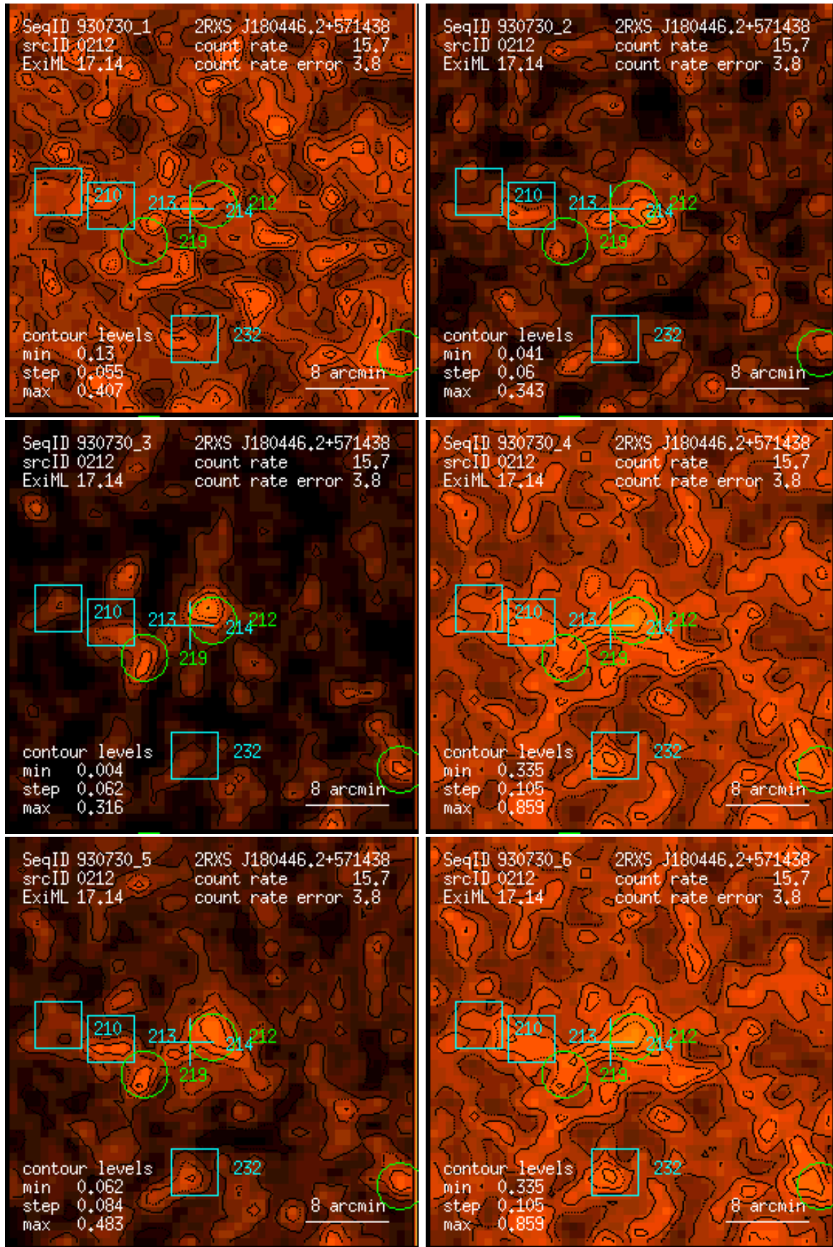
Figure 212: RASS 930730: detection 0212: band rate images, Gaussian filter: (1) PSPC channels 11 – 41, (2) 52 – 90, (3) 91 – 201, (4) 11 – 235, (5) 52 – 201, (6) 11 – 201. Broad band rates in counts/ks. Band rate contour levels in counts/ks/arcmin 2 .
