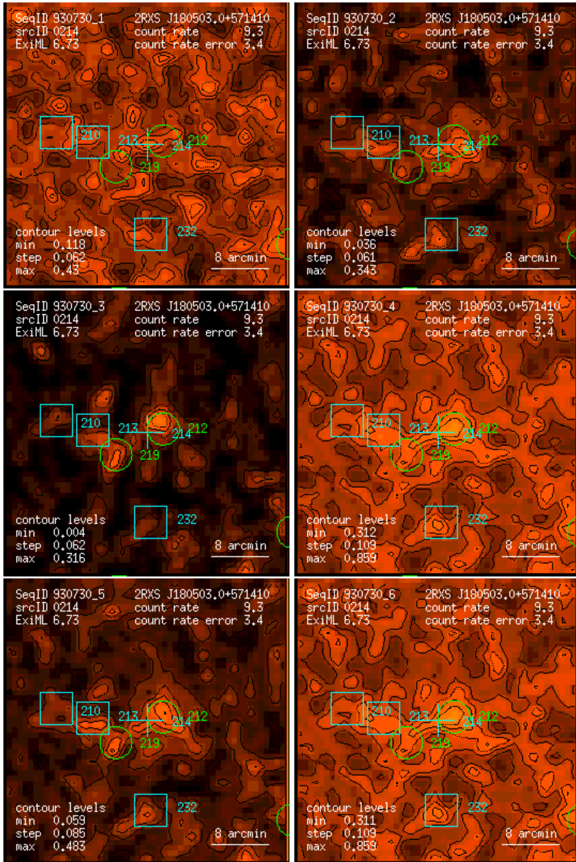
Figure 214: RASS 930730: detection 0214: band rate images, Gaussian filter: (1) PSPC channels 11 – 41, (2) 52 – 90, (3) 91 – 201, (4) 11 – 235, (5) 52 – 201, (6) 11 – 201. Broad band rates in counts/ks. Band rate contour levels in counts/ks/arcmin 2 .
