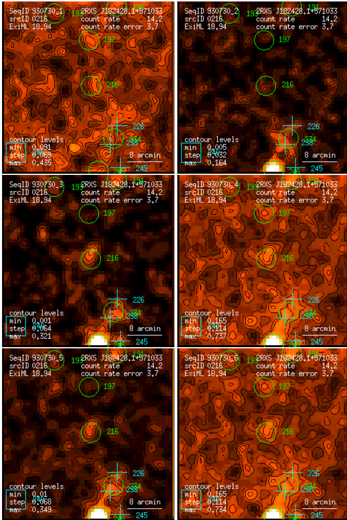
Figure 216: RASS 930730: detection 0216: band rate images, Gaussian filter: (1) PSPC channels 11 – 41, (2) 52 – 90, (3) 91 – 201, (4) 11 – 235, (5) 52 – 201, (6) 11 – 201. Broad band rates in counts/ks. Band rate contour levels in counts/ks/arcmin 2 .
