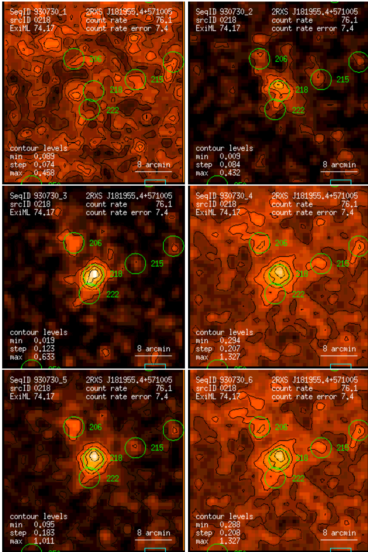
Figure 218: RASS 930730: detection 0218: band rate images, Gaussian filter: (1) PSPC channels 11 – 41, (2) 52 – 90, (3) 91 – 201, (4) 11 – 235, (5) 52 – 201, (6) 11 – 201. Broad band rates in counts/ks. Band rate contour levels in counts/ks/arcmin 2 .
