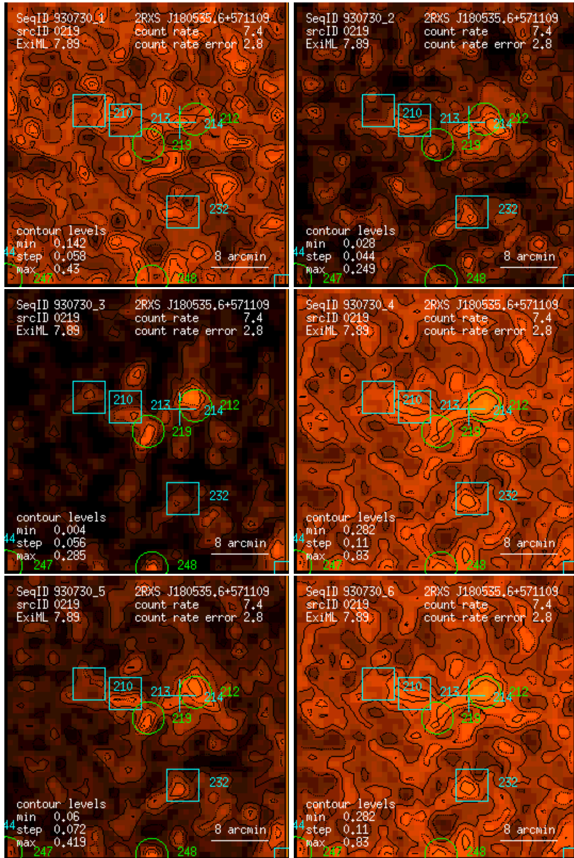
Figure 219: RASS 930730: detection 0219: band rate images, Gaussian filter: (1) PSPC channels 11 – 41, (2) 52 – 90, (3) 91 – 201, (4) 11 – 235, (5) 52 – 201, (6) 11 – 201. Broad band rates in counts/ks. Band rate contour levels in counts/ks/arcmin 2 .
