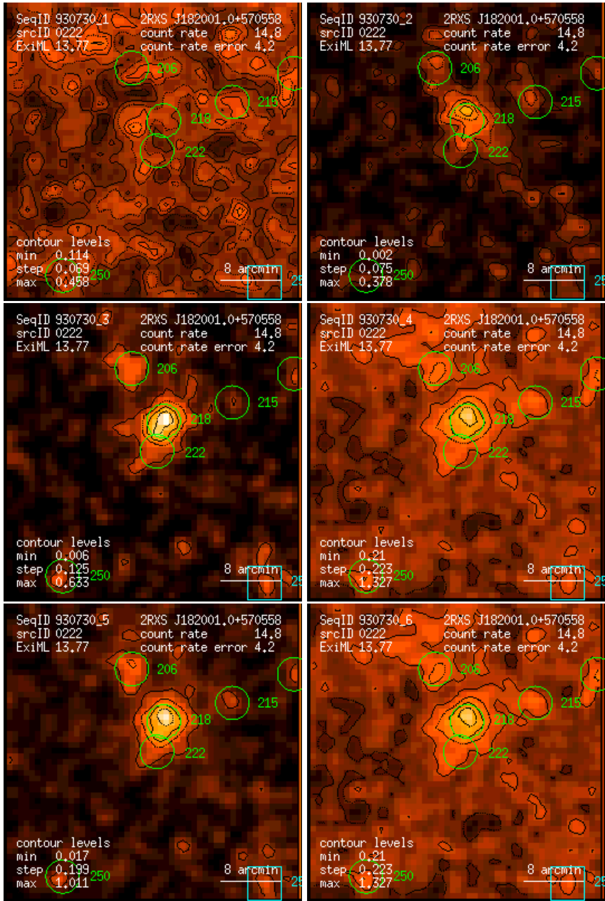
Figure 222: RASS 930730: detection 0222: band rate images, Gaussian filter: (1) PSPC channels 11 – 41, (2) 52 – 90, (3) 91 – 201, (4) 11 – 235, (5) 52 – 201, (6) 11 – 201. Broad band rates in counts/ks. Band rate contour levels in counts/ks/arcmin 2 .
