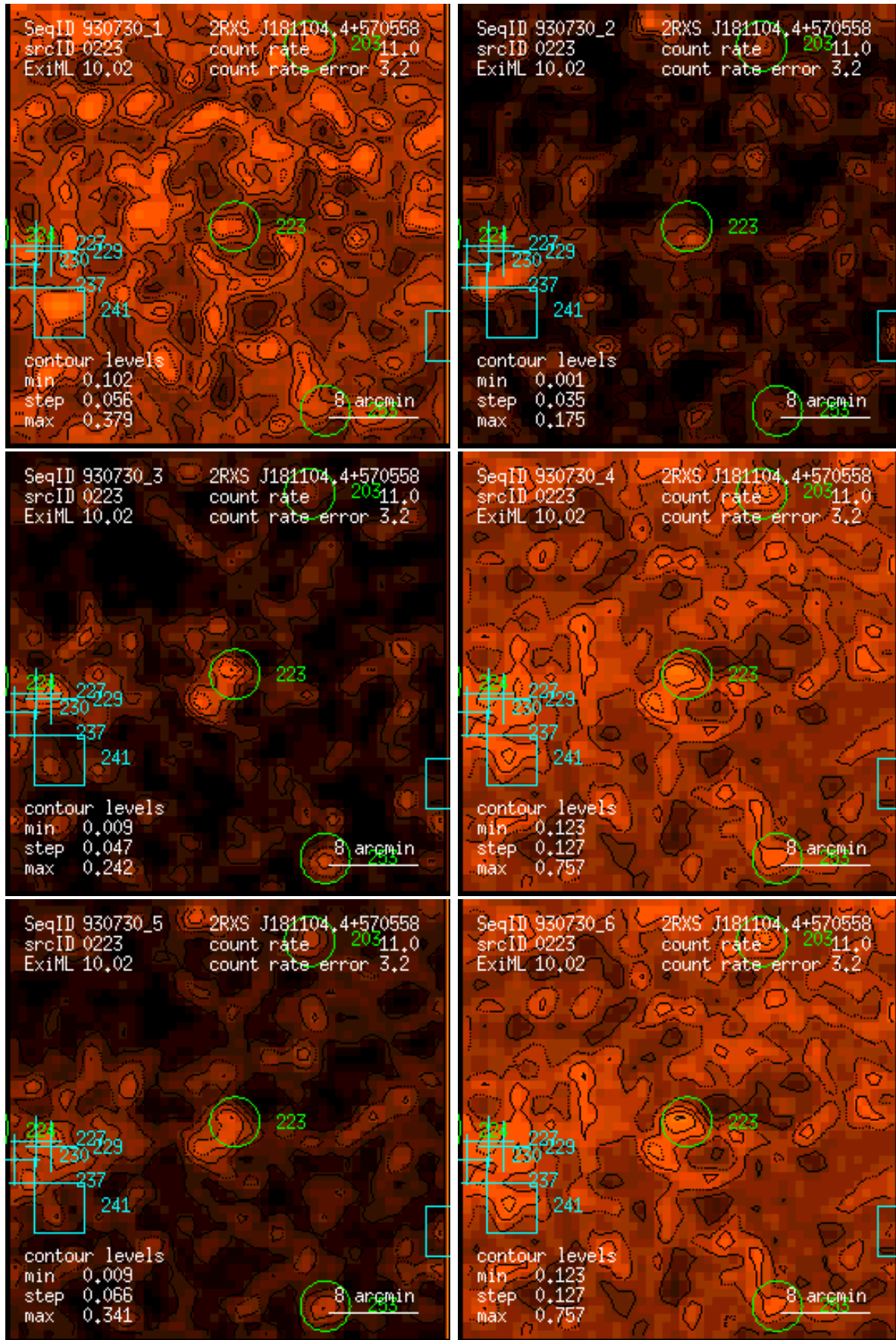
Figure 223: RASS 930730: detection 0223: band rate images, Gaussian filter: (1) PSPC channels 11 – 41, (2) 52 – 90, (3) 91 – 201, (4) 11 – 235, (5) 52 – 201, (6) 11 – 201. Broad band rates in counts/ks. Band rate contour levels in counts/ks/arcmin 2 .
