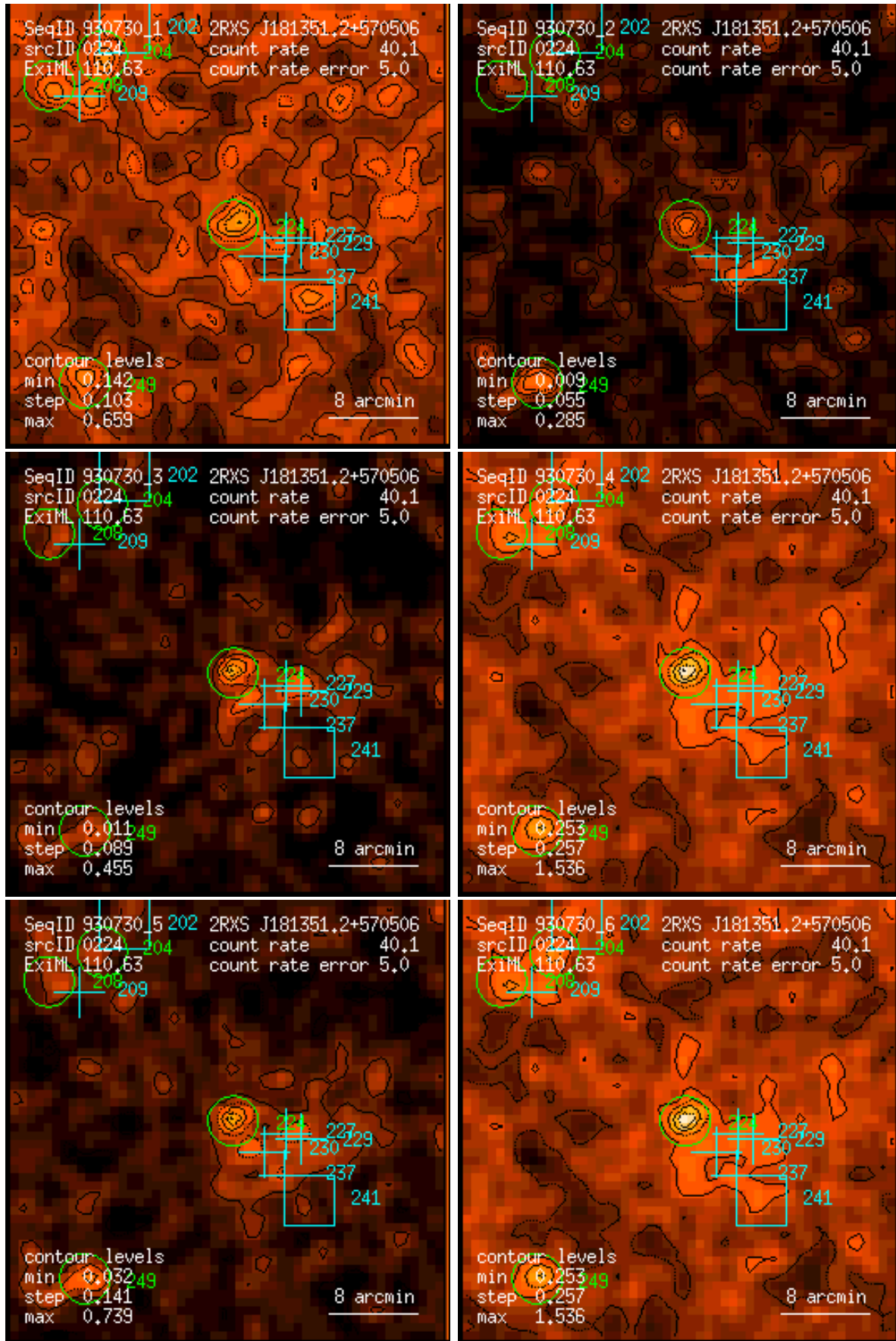
Figure 224: RASS 930730: detection 0224: band rate images, Gaussian filter: (1) PSPC channels 11 – 41, (2) 52 – 90, (3) 91 – 201, (4) 11 – 235, (5) 52 – 201, (6) 11 – 201. Broad band rates in counts/ks. Band rate contour levels in counts/ks/arcmin 2 .
