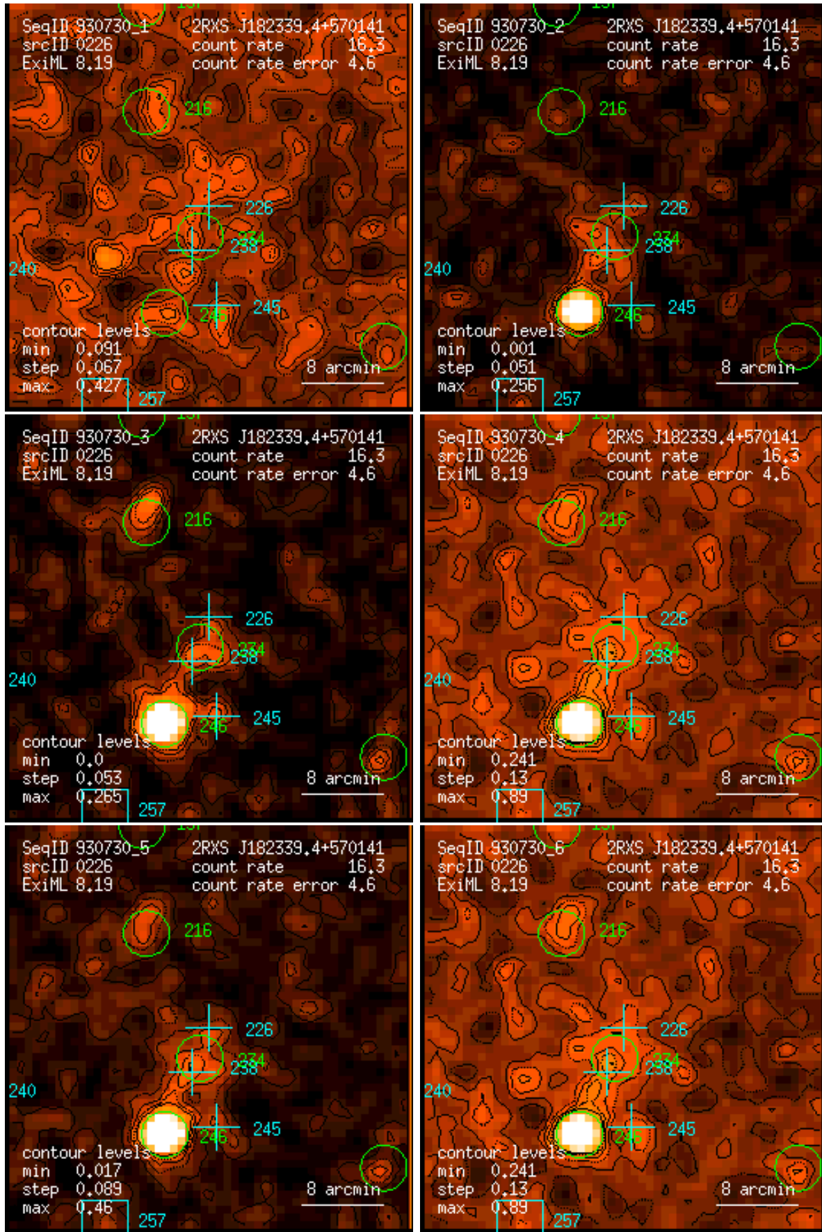
Figure 226: RASS 930730: detection 0226: band rate images, Gaussian filter: (1) PSPC channels 11 – 41, (2) 52 – 90, (3) 91 – 201, (4) 11 – 235, (5) 52 – 201, (6) 11 – 201. Broad band rates in counts/ks. Band rate contour levels in counts/ks/arcmin 2 .
