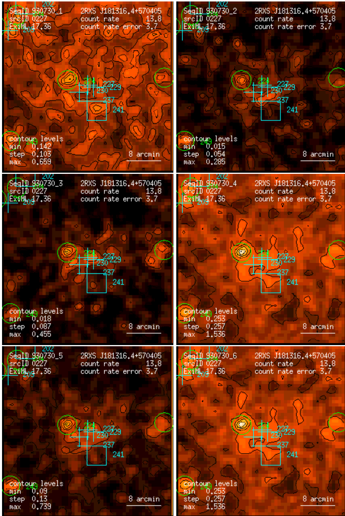
Figure 227: RASS 930730: detection 0227: band rate images, Gaussian filter: (1) PSPC channels 11 – 41, (2) 52 – 90, (3) 91 – 201, (4) 11 – 235, (5) 52 – 201, (6) 11 – 201. Broad band rates in counts/ks. Band rate contour levels in counts/ks/arcmin 2 .
