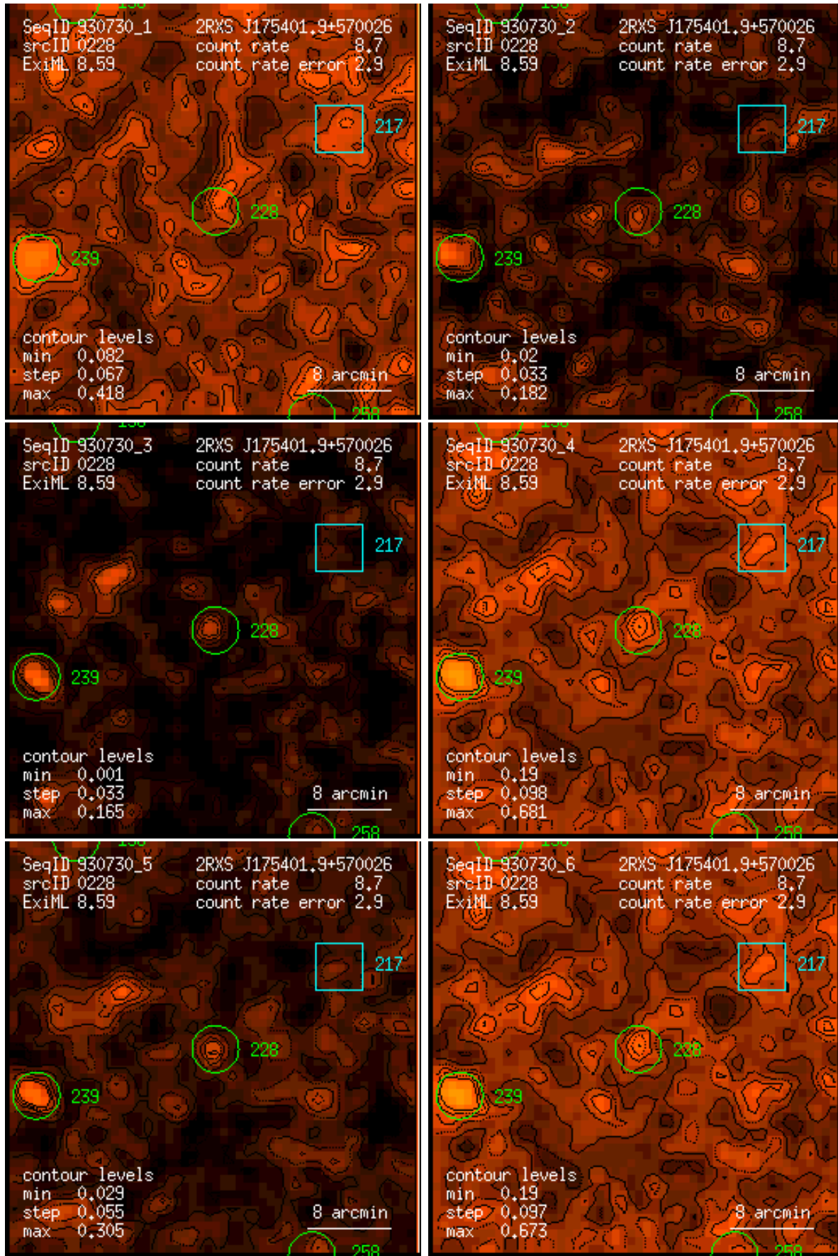
Figure 228: RASS 930730: detection 0228: band rate images, Gaussian filter: (1) PSPC channels 11 – 41, (2) 52 – 90, (3) 91 – 201, (4) 11 – 235, (5) 52 – 201, (6) 11 – 201. Broad band rates in counts/ks. Band rate contour levels in counts/ks/arcmin 2 .
