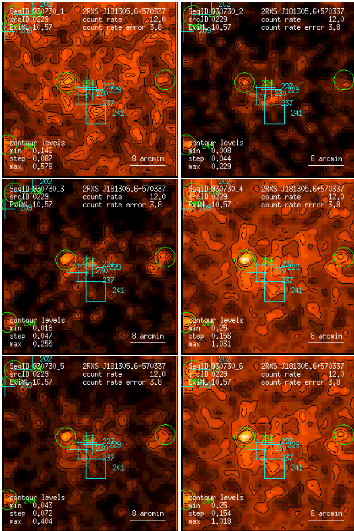
Figure 229: RASS 930730: detection 0229: band rate images, Gaussian filter: (1) PSPC channels 11 – 41, (2) 52 – 90, (3) 91 – 201, (4) 11 – 235, (5) 52 – 201, (6) 11 – 201. Broad band rates in counts/ks. Band rate contour levels in counts/ks/arcmin 2 .
