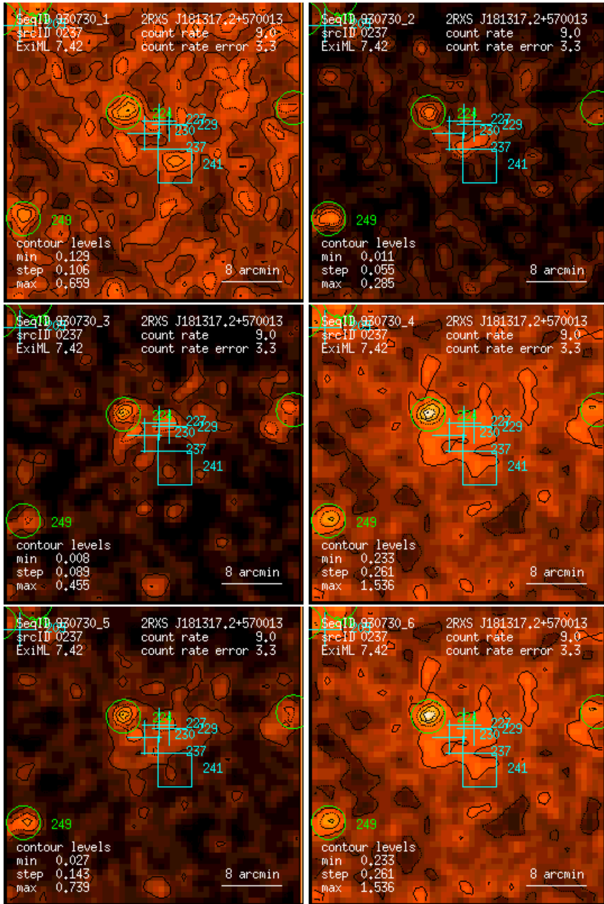
Figure 237: RASS 930730: detection 0237: band rate images, Gaussian filter: (1) PSPC channels 11 – 41, (2) 52 – 90, (3) 91 – 201, (4) 11 – 235, (5) 52 – 201, (6) 11 – 201. Broad band rates in counts/ks. Band rate contour levels in counts/ks/arcmin 2 .
