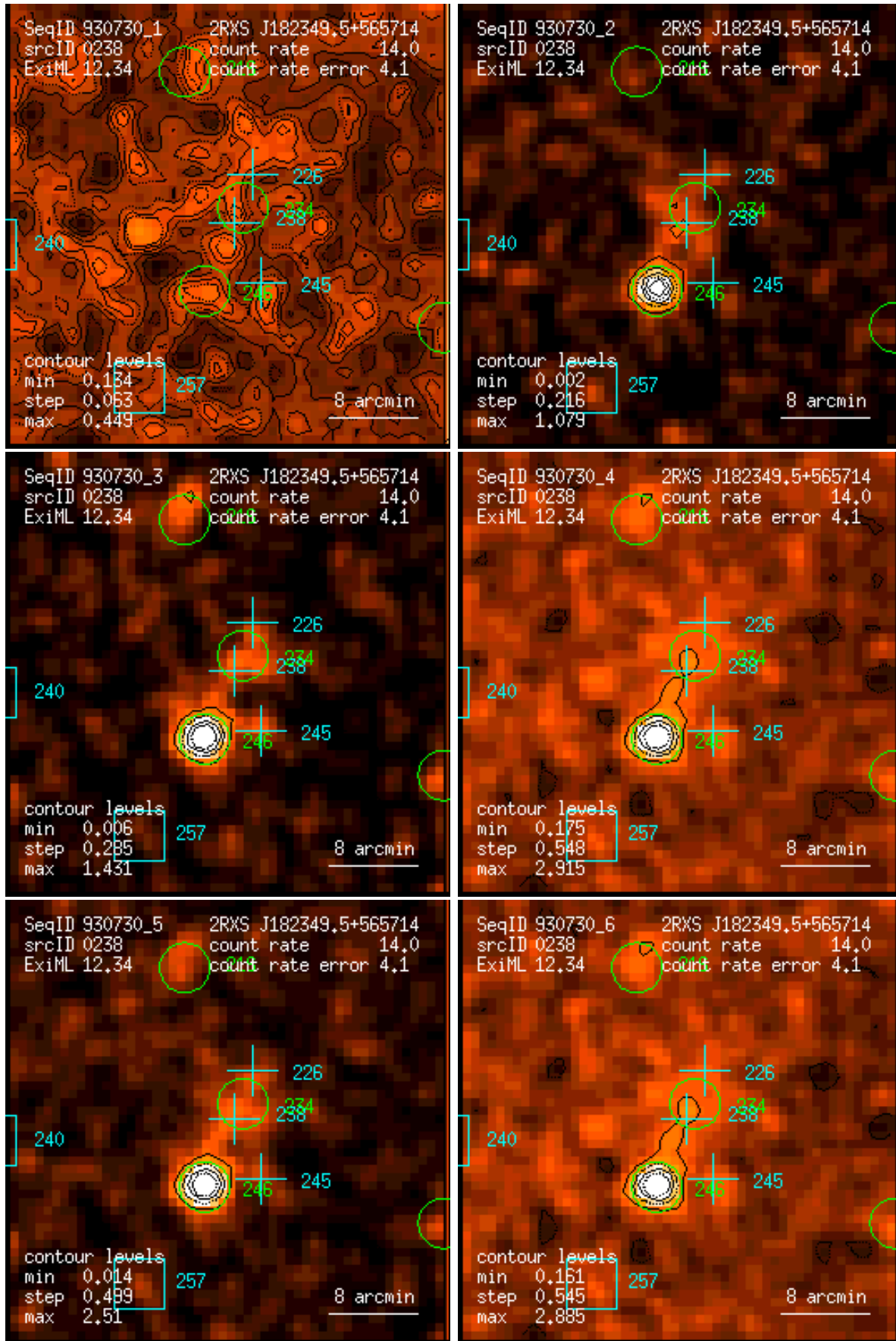
Figure 238: RASS 930730: detection 0238: band rate images, Gaussian filter: (1) PSPC channels 11 – 41, (2) 52 – 90, (3) 91 – 201, (4) 11 – 235, (5) 52 – 201, (6) 11 – 201. Broad band rates in counts/ks. Band rate contour levels in counts/ks/arcmin 2 .
