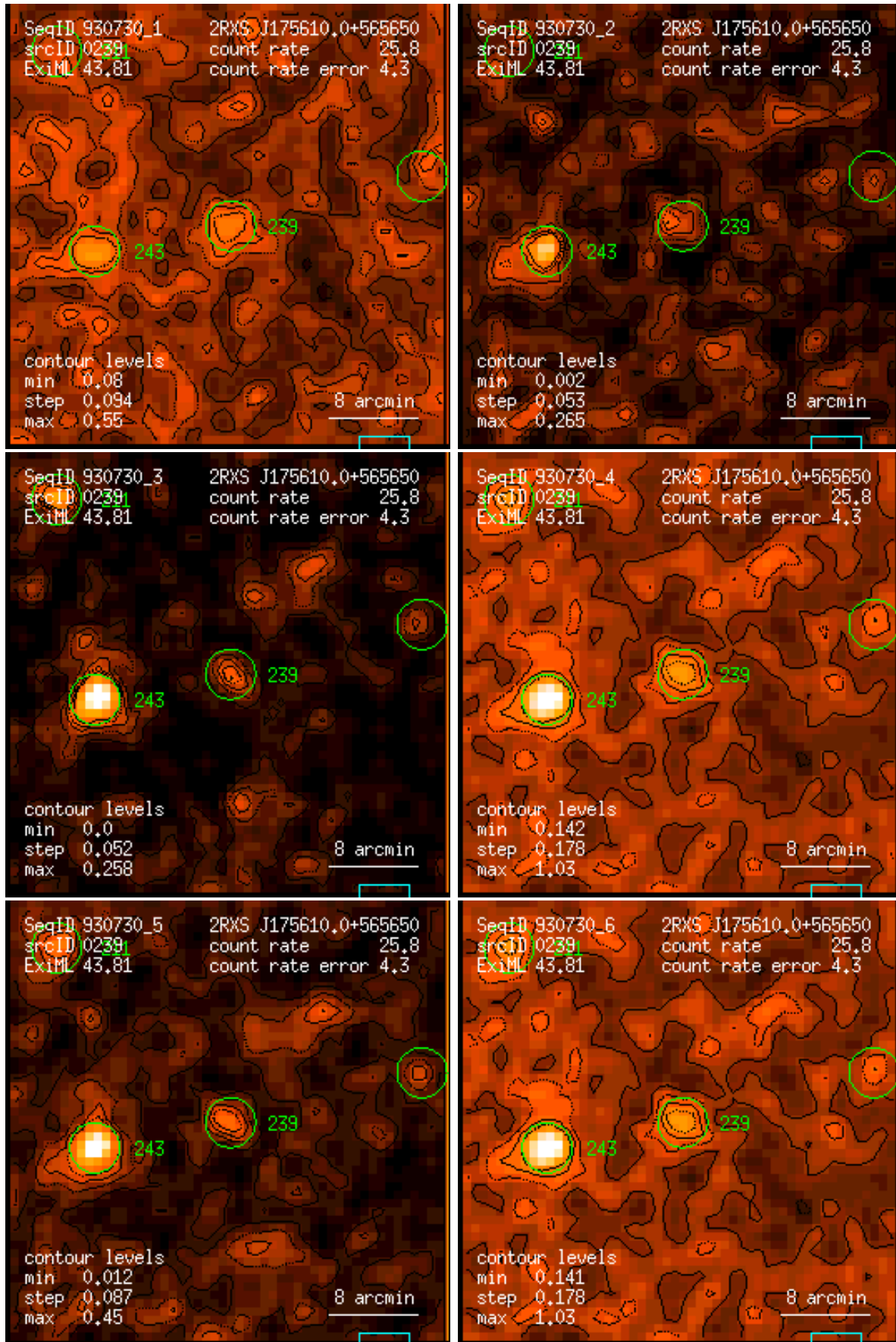
Figure 239: RASS 930730: detection 0239: band rate images, Gaussian filter: (1) PSPC channels 11 – 41, (2) 52 – 90, (3) 91 – 201, (4) 11 – 235, (5) 52 – 201, (6) 11 – 201. Broad band rates in counts/ks. Band rate contour levels in counts/ks/arcmin 2 .
