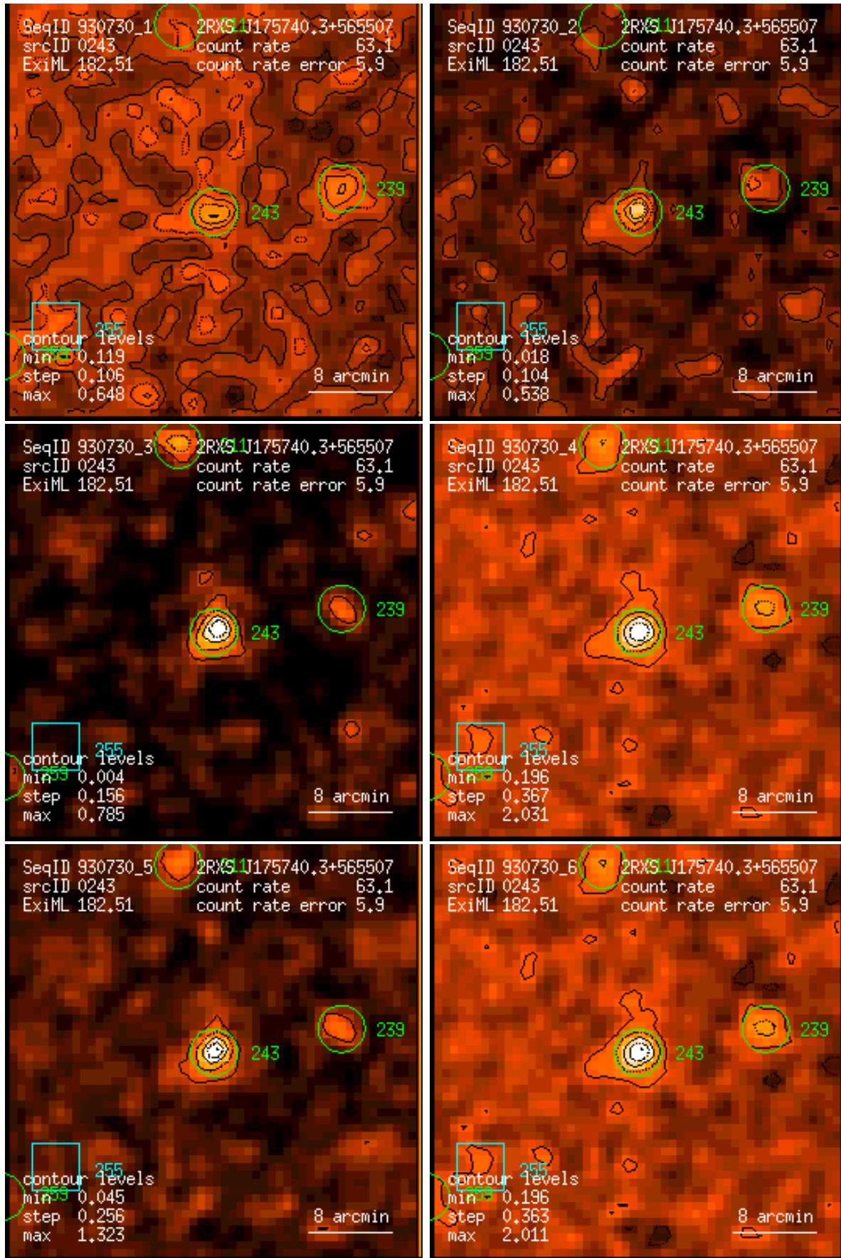
Figure 243: RASS 930730: detection 0243: band rate images, Gaussian filter: (1) PSPC channels 11 – 41, (2) 52 – 90, (3) 91 – 201, (4) 11 – 235, (5) 52 – 201, (6) 11 – 201. Broad band rates in counts/ks. Band rate contour levels in counts/ks/arcmin 2 .
