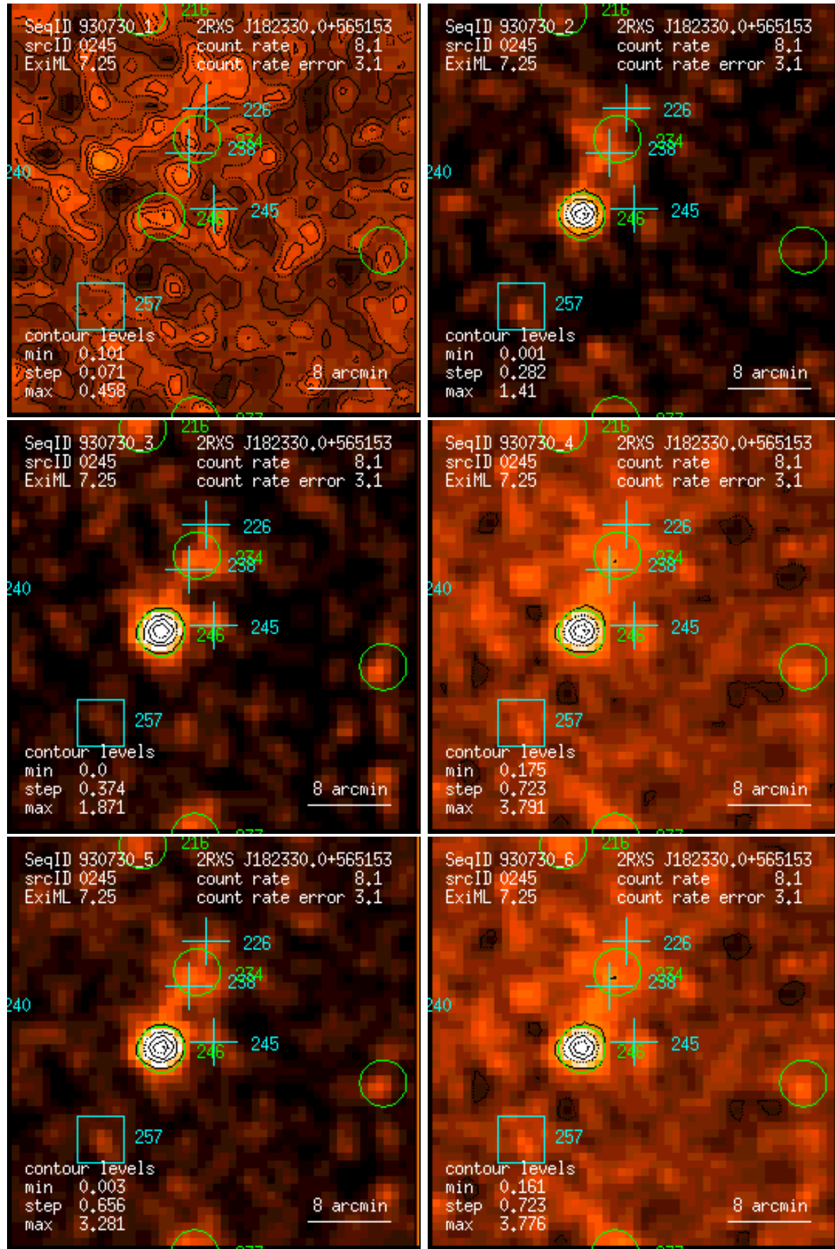
Figure 245: RASS 930730: detection 0245: band rate images, Gaussian filter: (1) PSPC channels 11 – 41, (2) 52 – 90, (3) 91 – 201, (4) 11 – 235, (5) 52 – 201, (6) 11 – 201. Broad band rates in counts/ks. Band rate contour levels in counts/ks/arcmin 2 .
