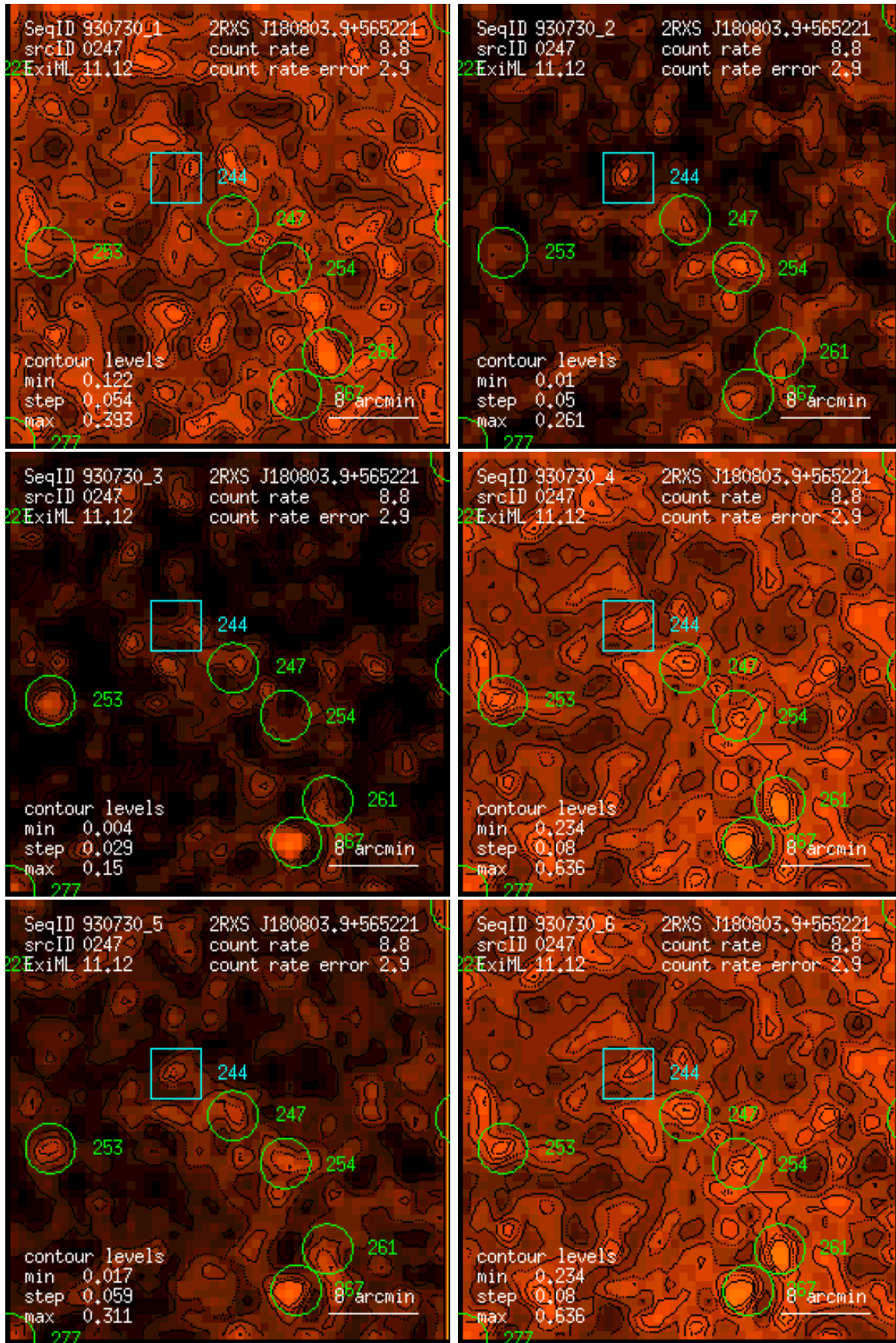
Figure 247: RASS 930730: detection 0247: band rate images, Gaussian filter: (1) PSPC channels 11 – 41, (2) 52 – 90, (3) 91 – 201, (4) 11 – 235, (5) 52 – 201, (6) 11 – 201. Broad band rates in counts/ks. Band rate contour levels in counts/ks/arcmin 2 .
