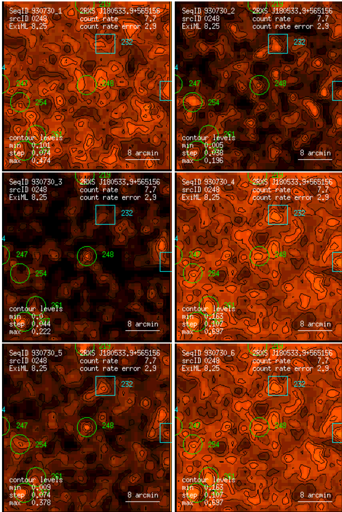
Figure 248: RASS 930730: detection 0248: band rate images, Gaussian filter: (1) PSPC channels 11 – 41, (2) 52 – 90, (3) 91 – 201, (4) 11 – 235, (5) 52 – 201, (6) 11 – 201. Broad band rates in counts/ks. Band rate contour levels in counts/ks/arcmin 2 .
