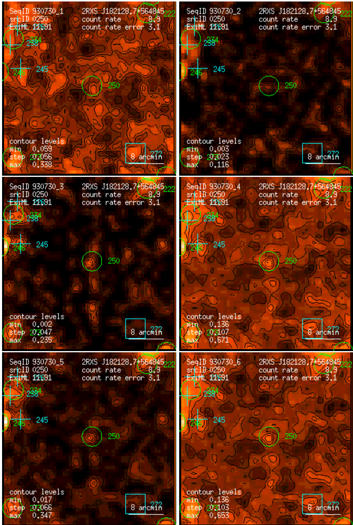
Figure 250: RASS 930730: detection 0250: band rate images, Gaussian filter: (1) PSPC channels 11 – 41, (2) 52 – 90, (3) 91 – 201, (4) 11 – 235, (5) 52 – 201, (6) 11 – 201. Broad band rates in counts/ks. Band rate contour levels in counts/ks/arcmin 2 .
