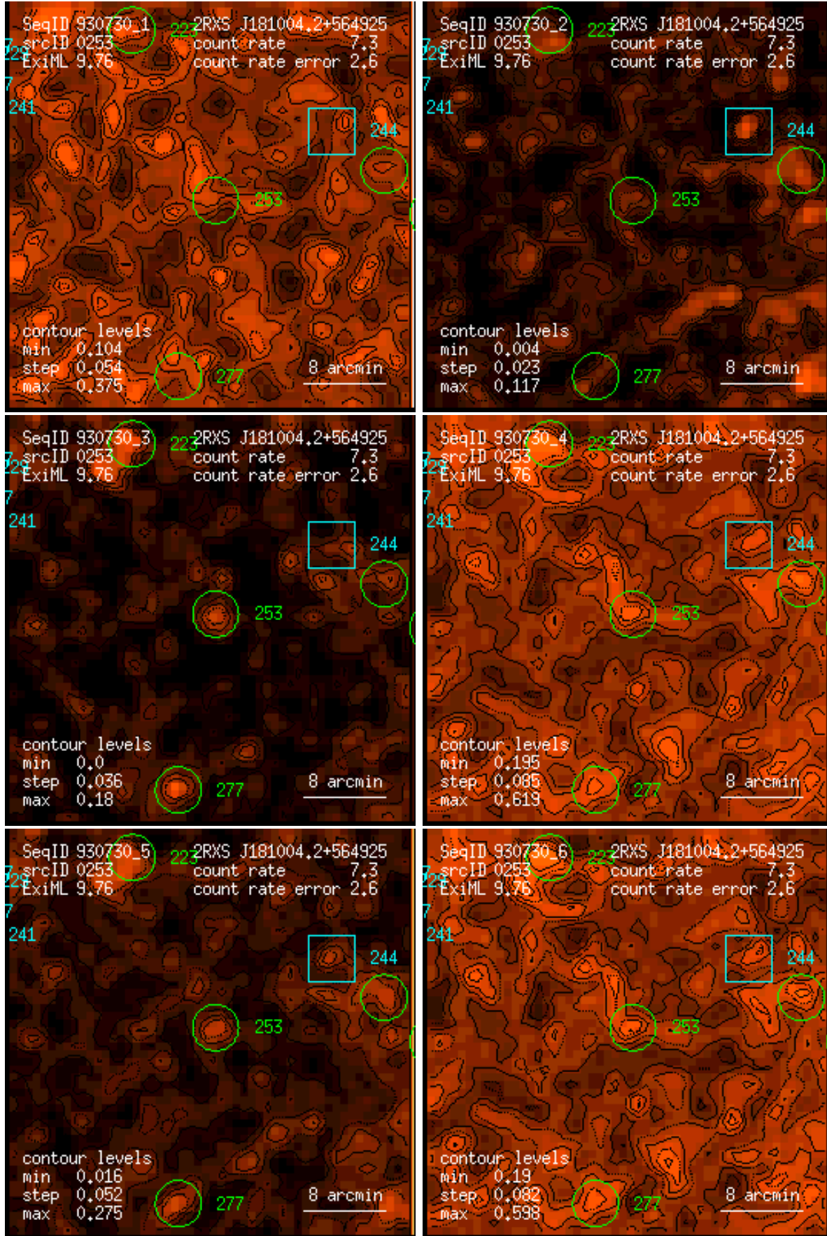
Figure 253: RASS 930730: detection 0253: band rate images, Gaussian filter: (1) PSPC channels 11 – 41, (2) 52 – 90, (3) 91 – 201, (4) 11 – 235, (5) 52 – 201, (6) 11 – 201. Broad band rates in counts/ks. Band rate contour levels in counts/ks/arcmin 2 .
