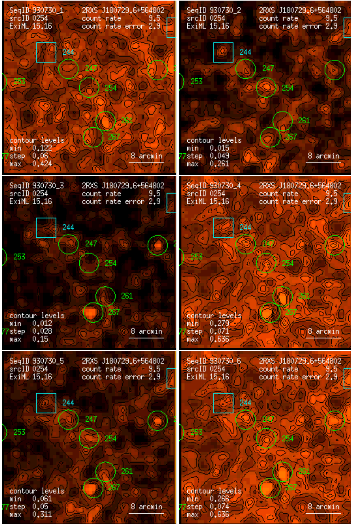
Figure 254: RASS 930730: detection 0254: band rate images, Gaussian filter: (1) PSPC channels 11 – 41, (2) 52 – 90, (3) 91 – 201, (4) 11 – 235, (5) 52 – 201, (6) 11 – 201. Broad band rates in counts/ks. Band rate contour levels in counts/ks/arcmin 2 .
