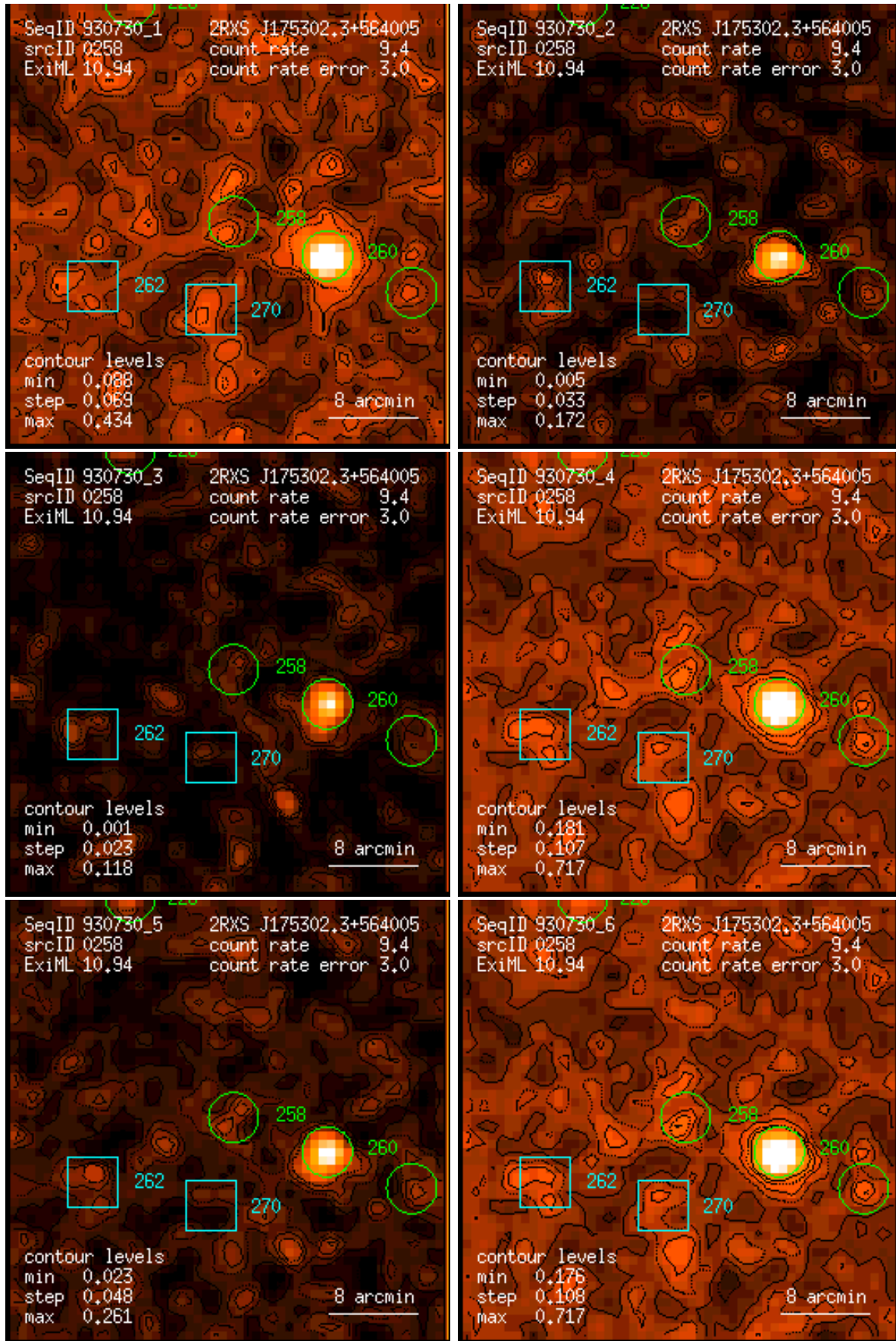
Figure 258: RASS 930730: detection 0258: band rate images, Gaussian filter: (1) PSPC channels 11 – 41, (2) 52 – 90, (3) 91 – 201, (4) 11 – 235, (5) 52 – 201, (6) 11 – 201. Broad band rates in counts/ks. Band rate contour levels in counts/ks/arcmin 2 .
