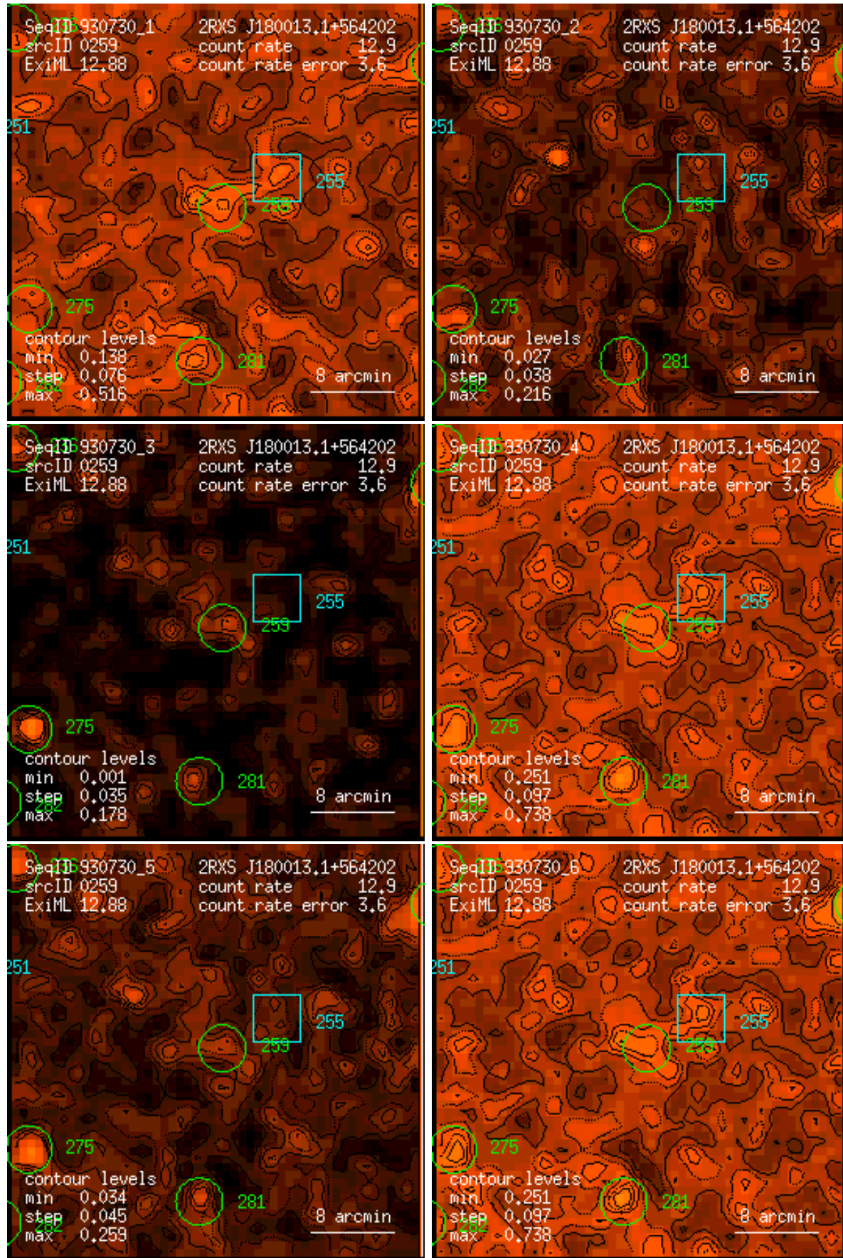
Figure 259: RASS 930730: detection 0259: band rate images, Gaussian filter: (1) PSPC channels 11 – 41, (2) 52 – 90, (3) 91 – 201, (4) 11 – 235, (5) 52 – 201, (6) 11 – 201. Broad band rates in counts/ks. Band rate contour levels in counts/ks/arcmin 2 .
