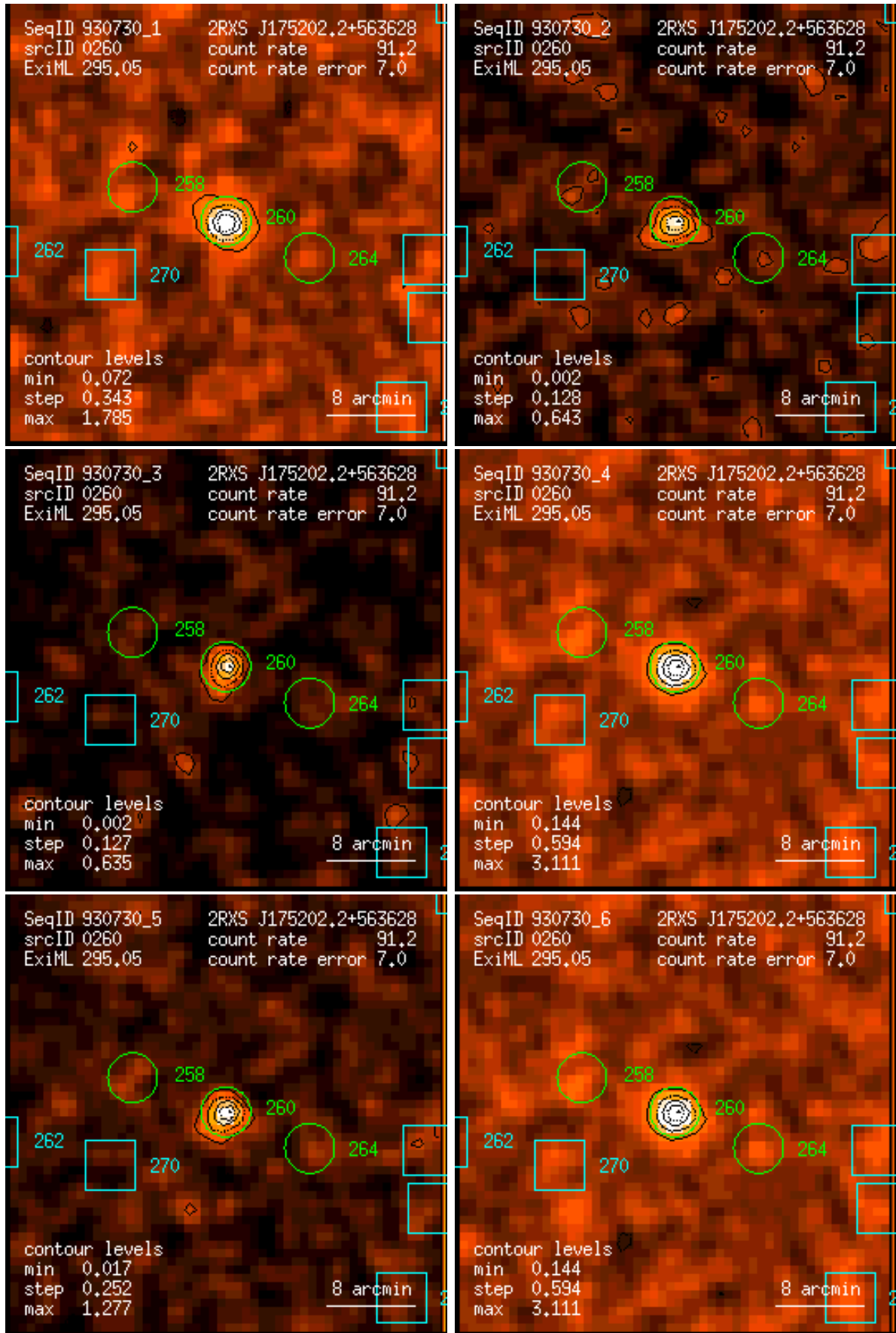
Figure 260: RASS 930730: detection 0260: band rate images, Gaussian filter: (1) PSPC channels 11 – 41, (2) 52 – 90, (3) 91 – 201, (4) 11 – 235, (5) 52 – 201, (6) 11 – 201. Broad band rates in counts/ks. Band rate contour levels in counts/ks/arcmin 2 .
