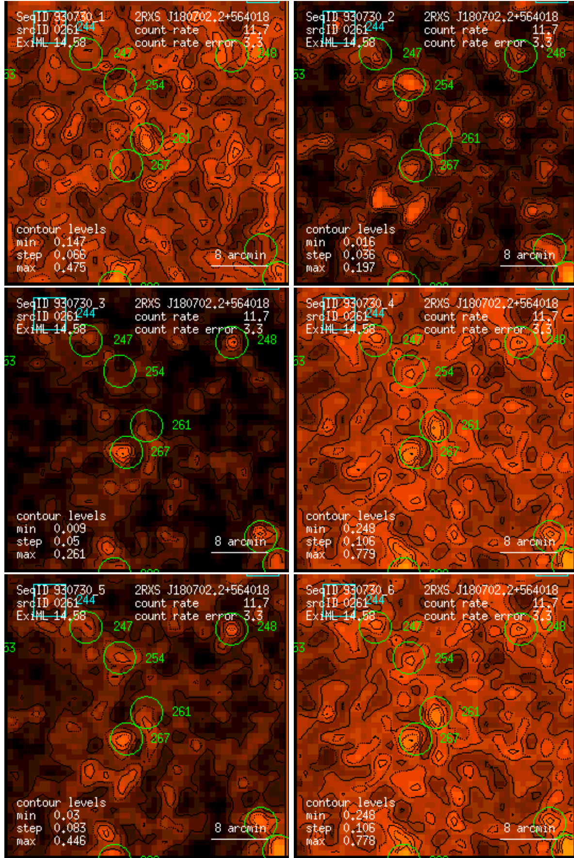
Figure 261: RASS 930730: detection 0261: band rate images, Gaussian filter: (1) PSPC channels 11 – 41, (2) 52 – 90, (3) 91 – 201, (4) 11 – 235, (5) 52 – 201, (6) 11 – 201. Broad band rates in counts/ks. Band rate contour levels in counts/ks/arcmin 2 .
