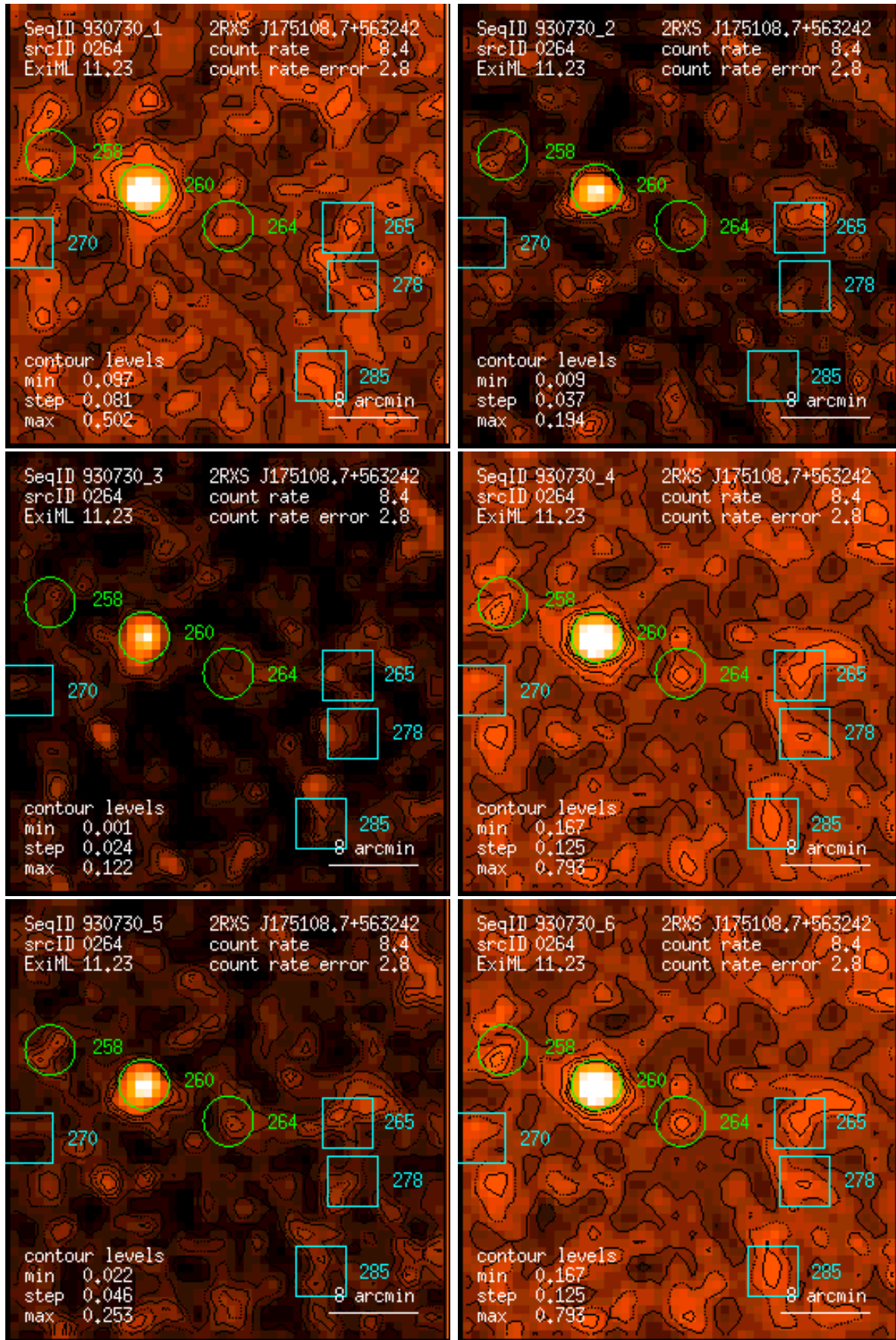
Figure 264: RASS 930730: detection 0264: band rate images, Gaussian filter: (1) PSPC channels 11 – 41, (2) 52 – 90, (3) 91 – 201, (4) 11 – 235, (5) 52 – 201, (6) 11 – 201. Broad band rates in counts/ks. Band rate contour levels in counts/ks/arcmin 2 .
