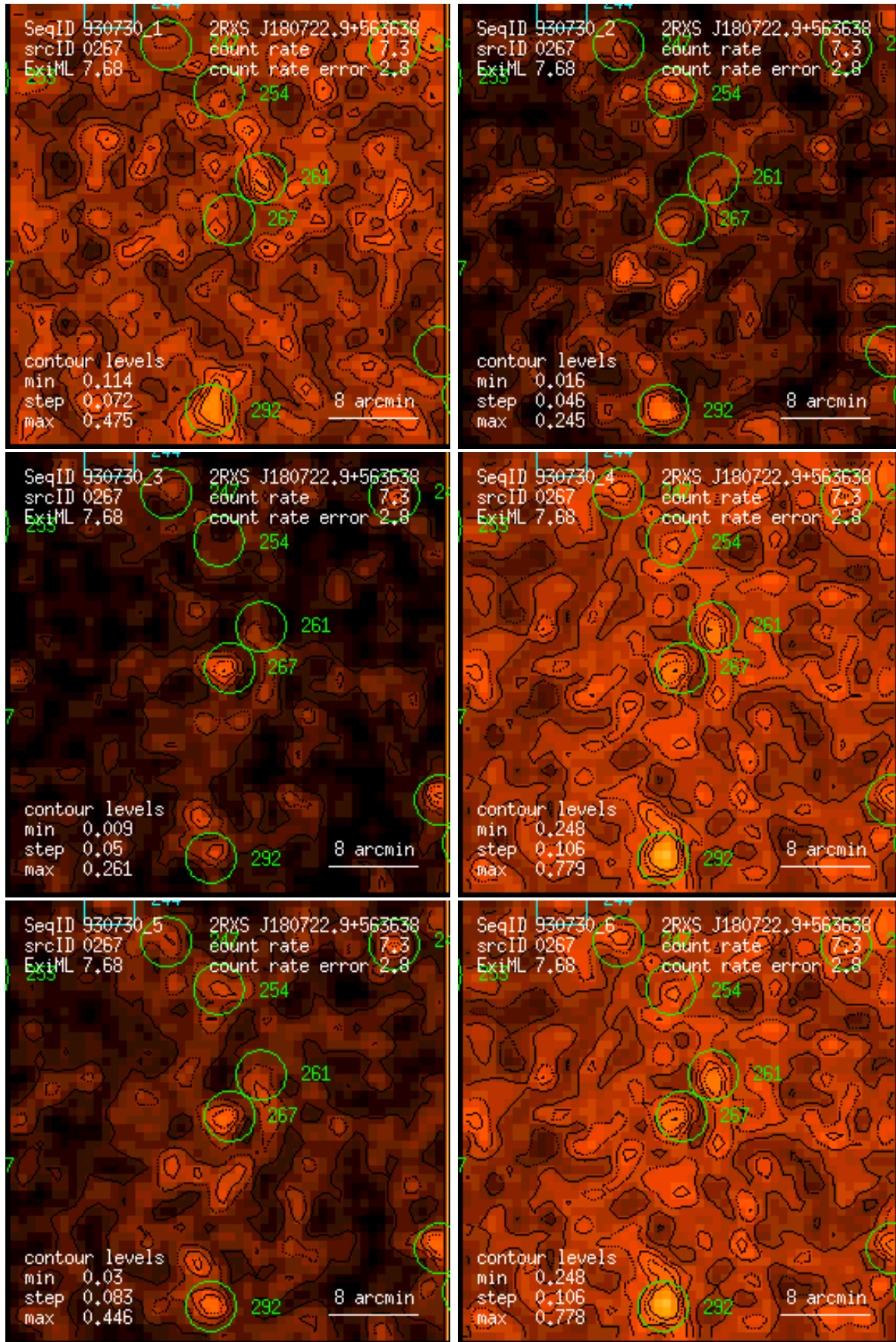
Figure 267: RASS 930730: detection 0267: band rate images, Gaussian filter: (1) PSPC channels 11 – 41, (2) 52 – 90, (3) 91 – 201, (4) 11 – 235, (5) 52 – 201, (6) 11 – 201. Broad band rates in counts/ks. Band rate contour levels in counts/ks/arcmin 2 .
