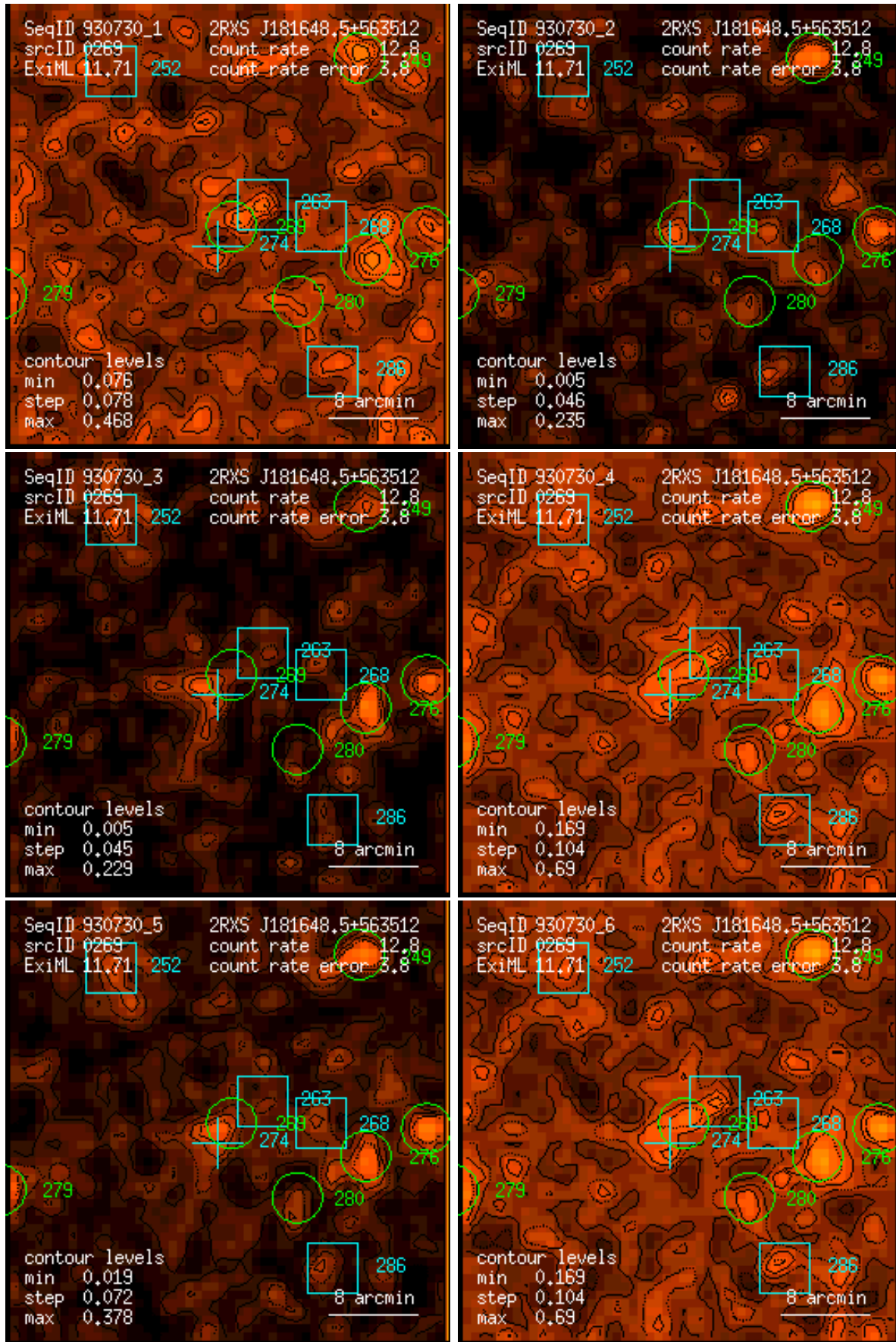
Figure 269: RASS 930730: detection 0269: band rate images, Gaussian filter: (1) PSPC channels 11 – 41, (2) 52 – 90, (3) 91 – 201, (4) 11 – 235, (5) 52 – 201, (6) 11 – 201. Broad band rates in counts/ks. Band rate contour levels in counts/ks/arcmin 2 .
