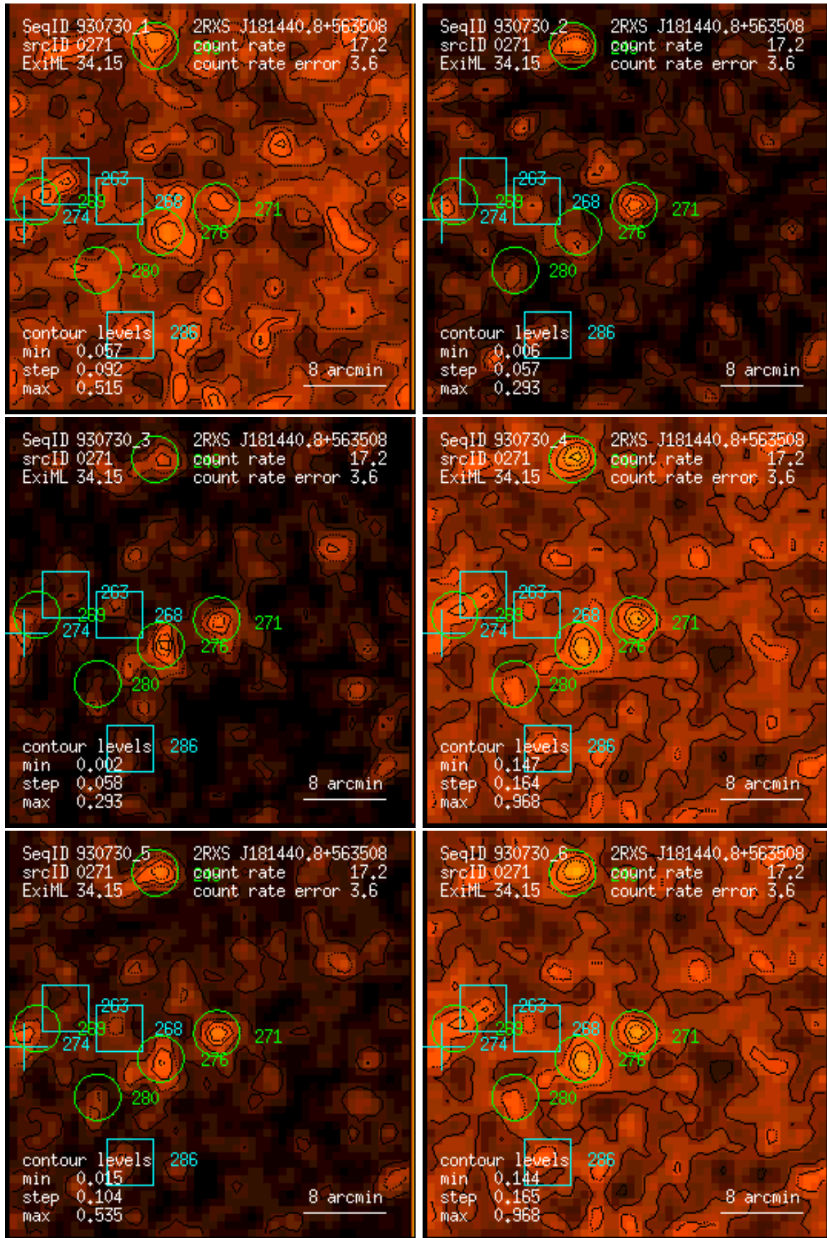
Figure 271: RASS 930730: detection 0271: band rate images, Gaussian filter: (1) PSPC channels 11 – 41, (2) 52 – 90, (3) 91 – 201, (4) 11 – 235, (5) 52 – 201, (6) 11 – 201. Broad band rates in counts/ks. Band rate contour levels in counts/ks/arcmin 2 .
