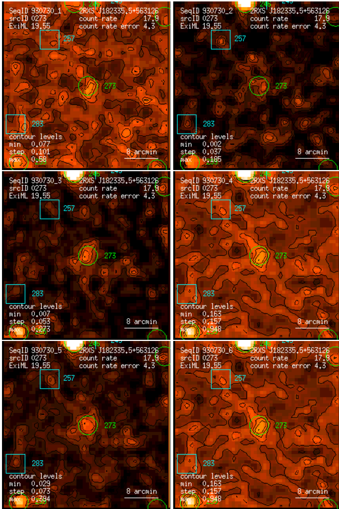
Figure 273: RASS 930730: detection 0273: band rate images, Gaussian filter: (1) PSPC channels 11 – 41, (2) 52 – 90, (3) 91 – 201, (4) 11 – 235, (5) 52 – 201, (6) 11 – 201. Broad band rates in counts/ks. Band rate contour levels in counts/ks/arcmin 2 .
