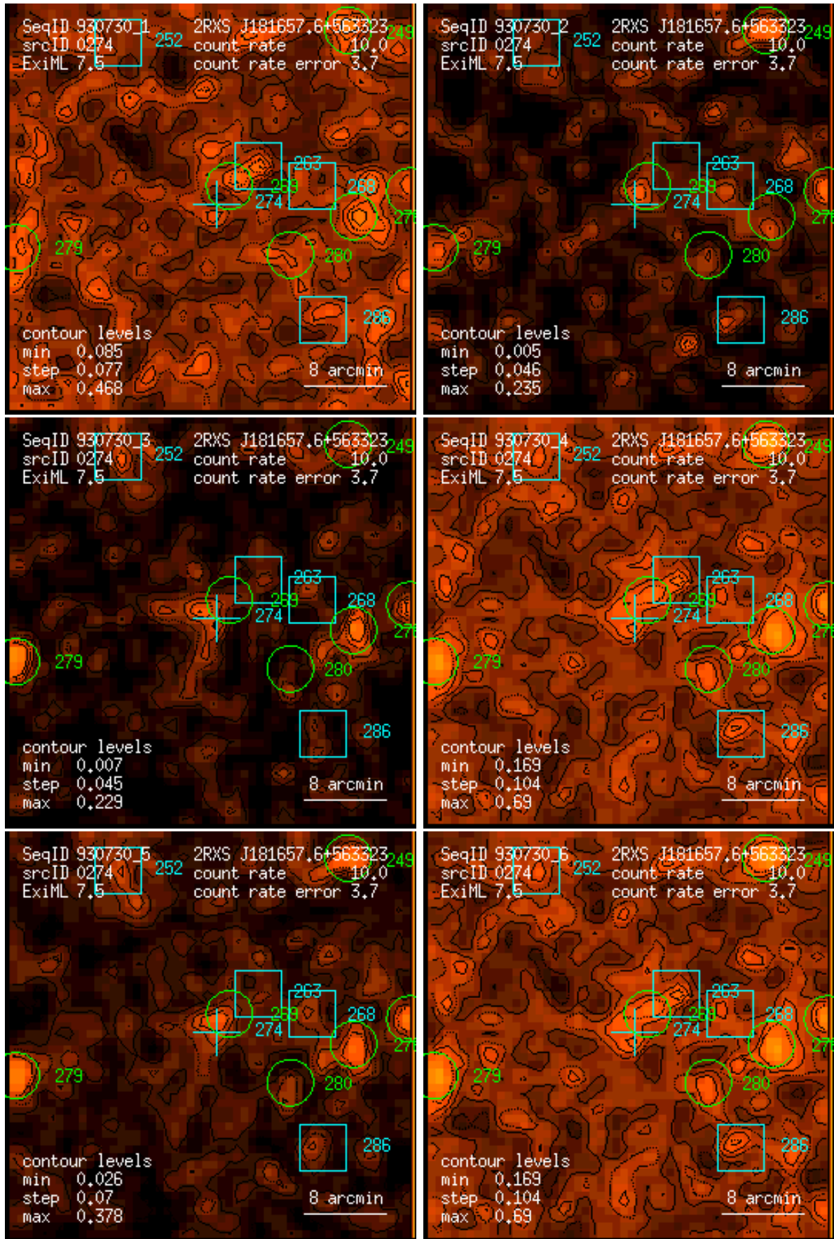
Figure 274: RASS 930730: detection 0274: band rate images, Gaussian filter: (1) PSPC channels 11 – 41, (2) 52 – 90, (3) 91 – 201, (4) 11 – 235, (5) 52 – 201, (6) 11 – 201. Broad band rates in counts/ks. Band rate contour levels in counts/ks/arcmin 2 .
