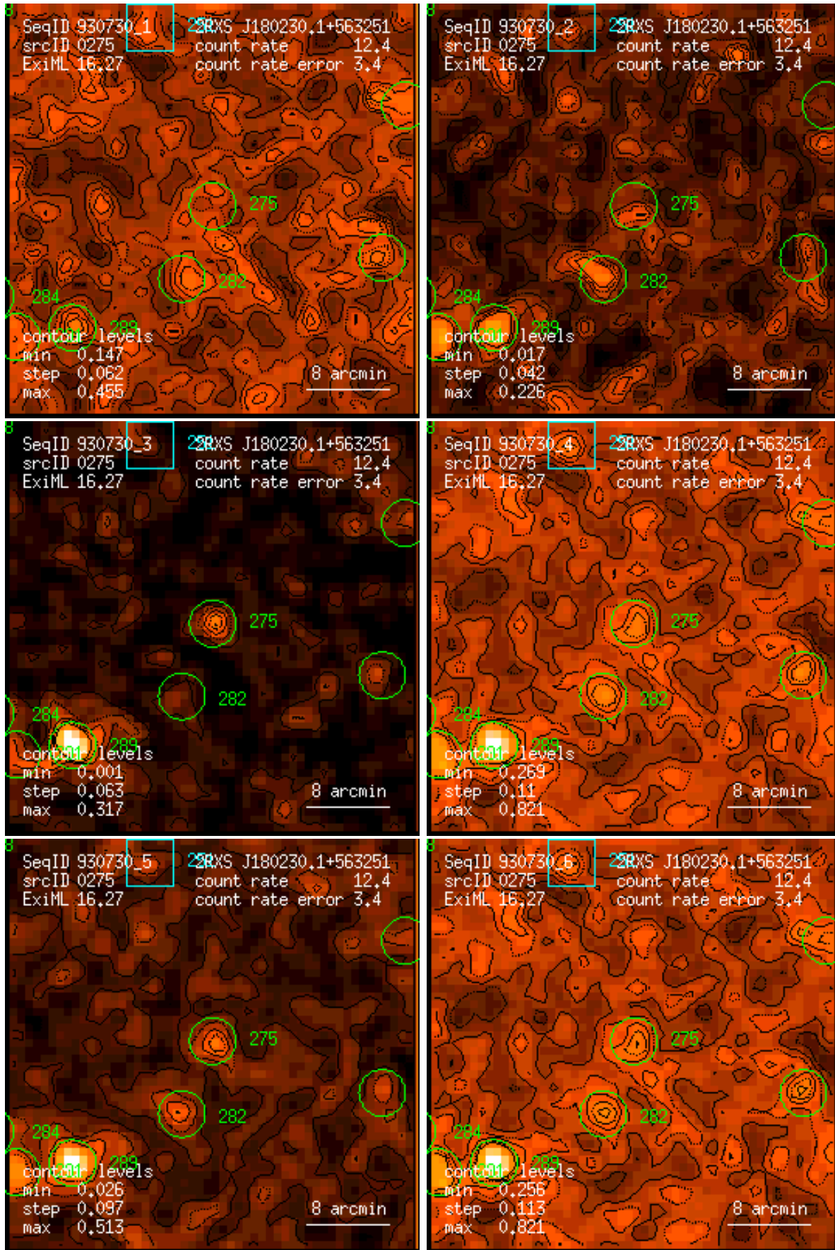
Figure 275: RASS 930730: detection 0275: band rate images, Gaussian filter: (1) PSPC channels 11 – 41, (2) 52 – 90, (3) 91 – 201, (4) 11 – 235, (5) 52 – 201, (6) 11 – 201. Broad band rates in counts/ks. Band rate contour levels in counts/ks/arcmin 2 .
